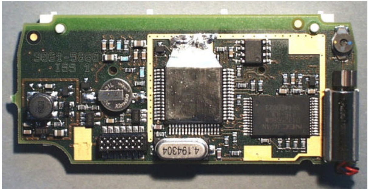
TLA852/FLA872 - DECODER PCB REAR VIEW
