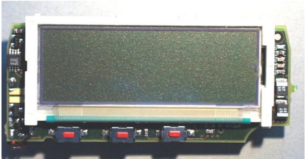
TLA852/FLA872 - DECODER PCB FRONT VIEW
