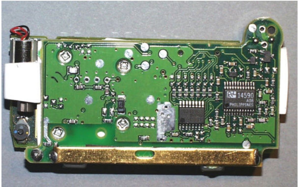
TLA852/FLA872 - RADIO REAR VIEW
