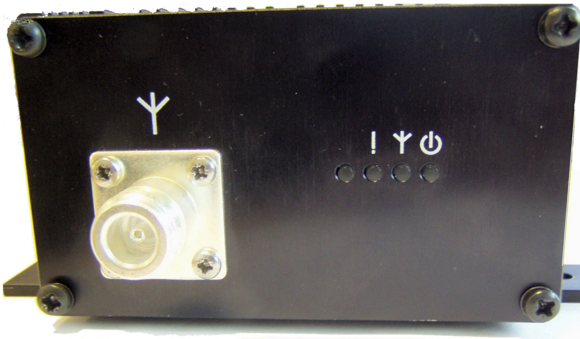
RPT 503 RF Connector End-plate Detail
