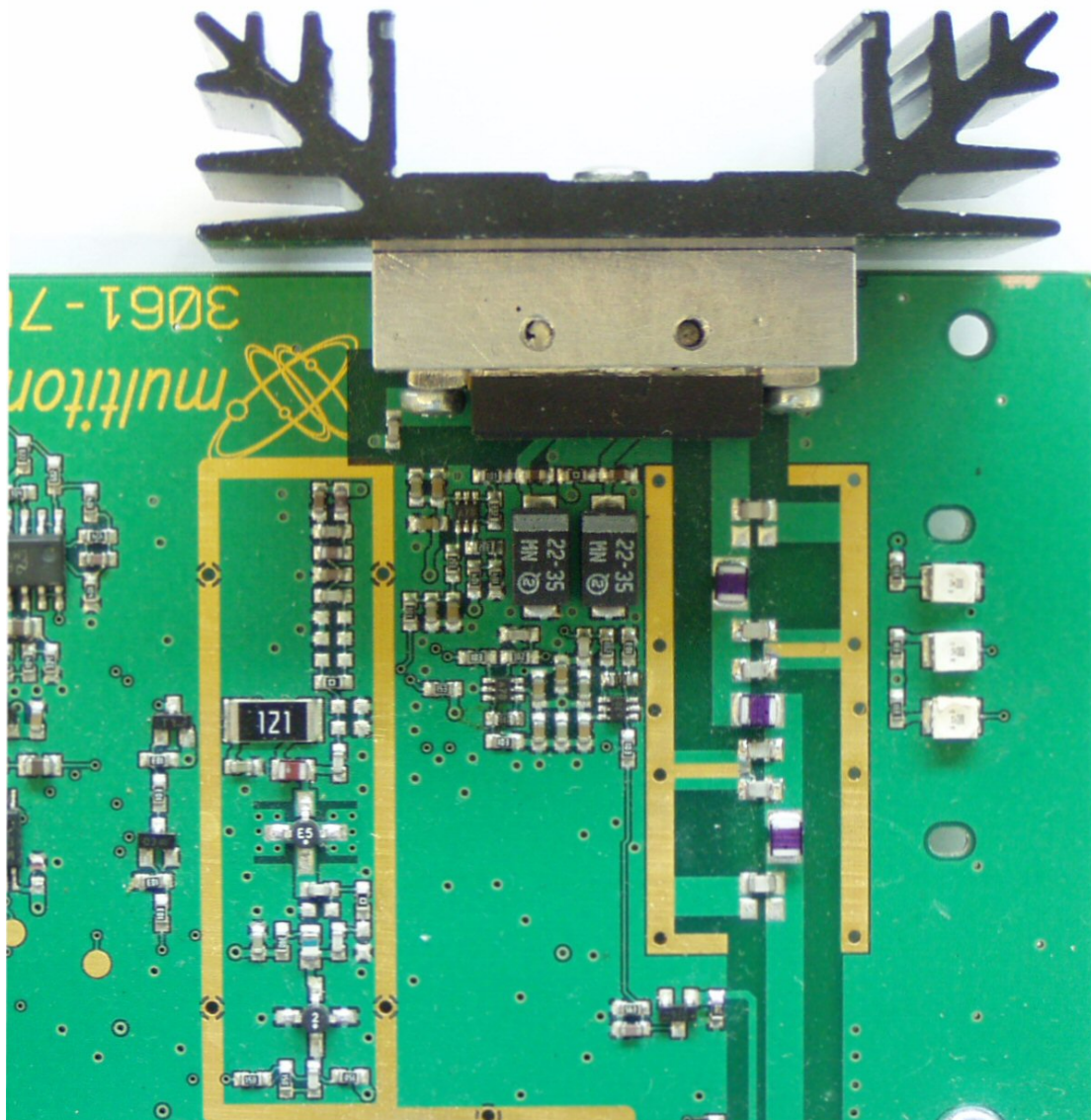
RPE/RPT 503 Detail Of RF PA Stage
