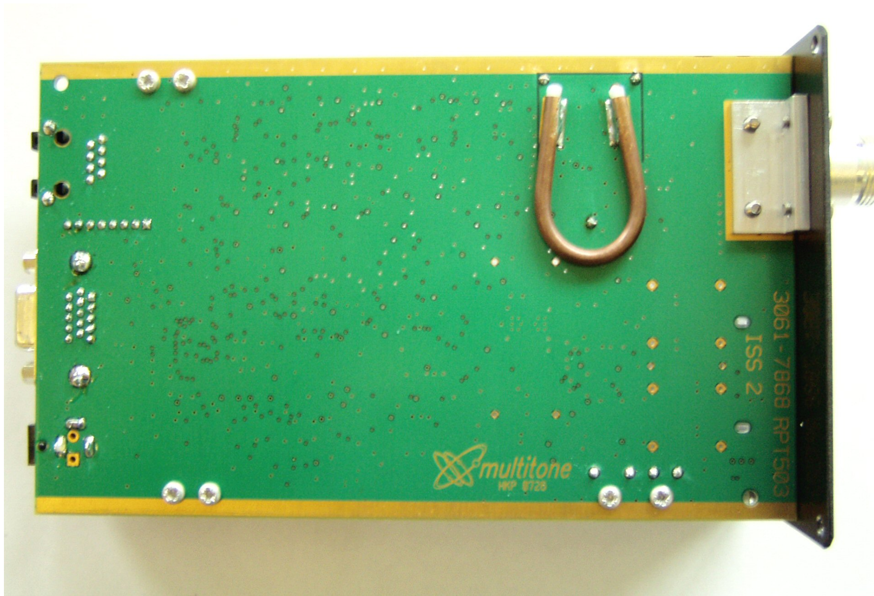
RPT 503 PCB Underside
