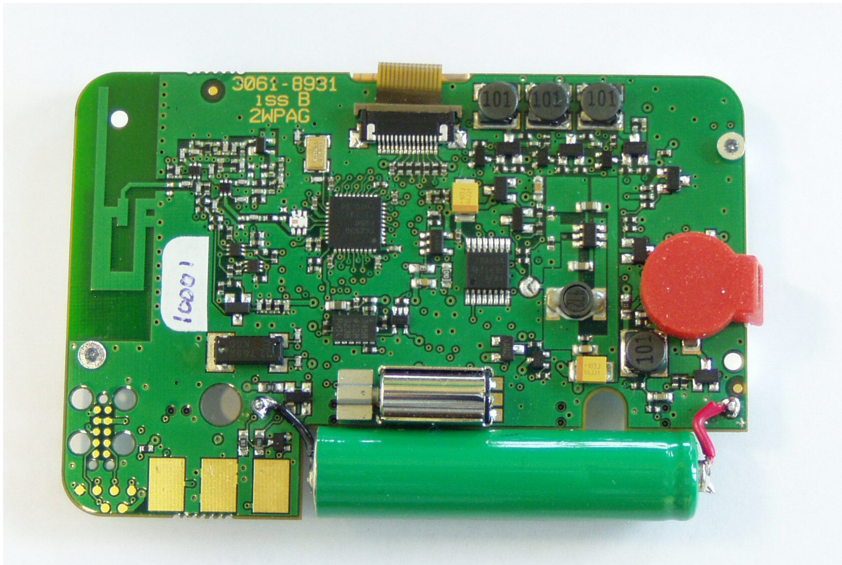
EKOPAG – PCB Underside
