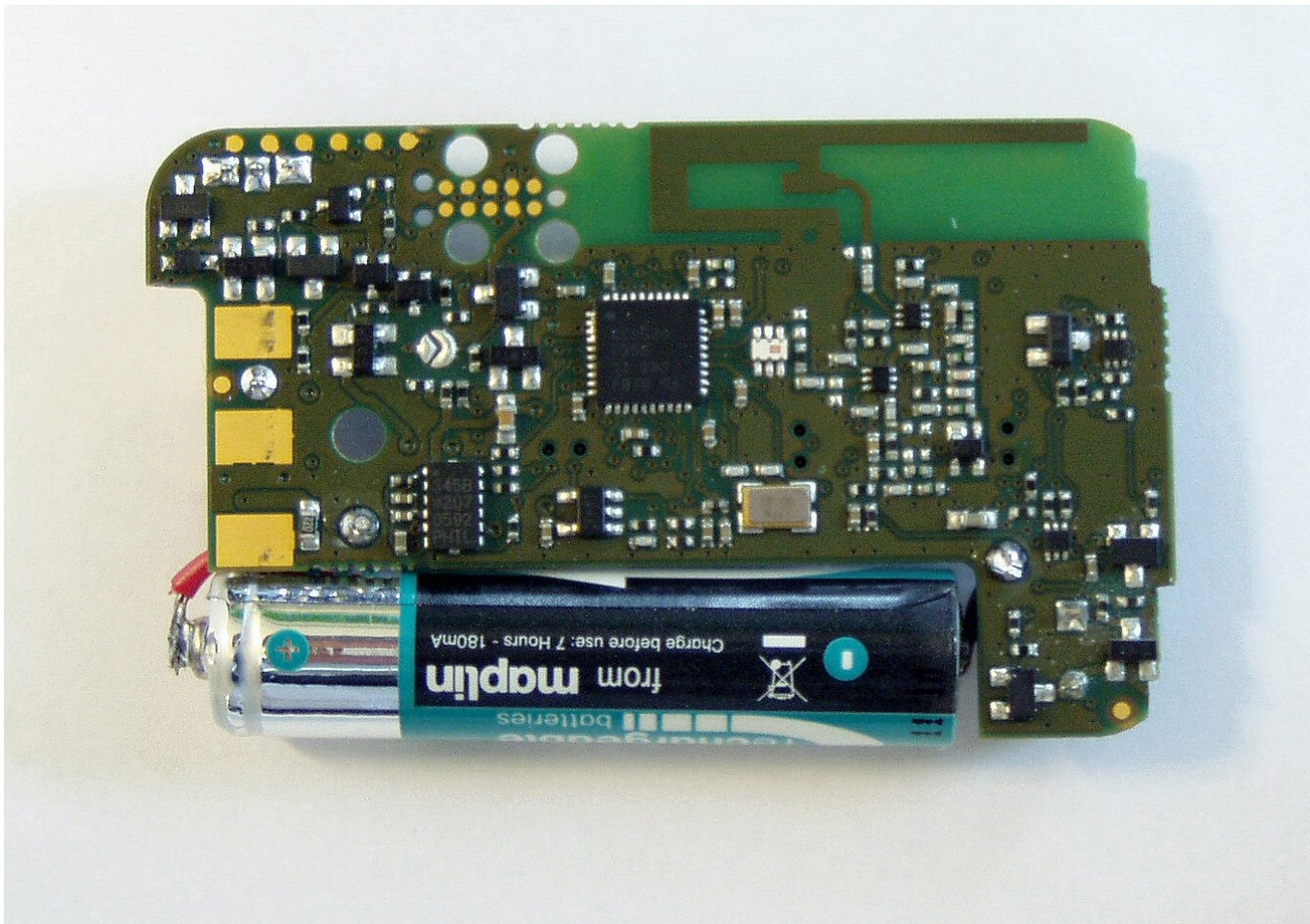
EKOFOB – PCB Underside
