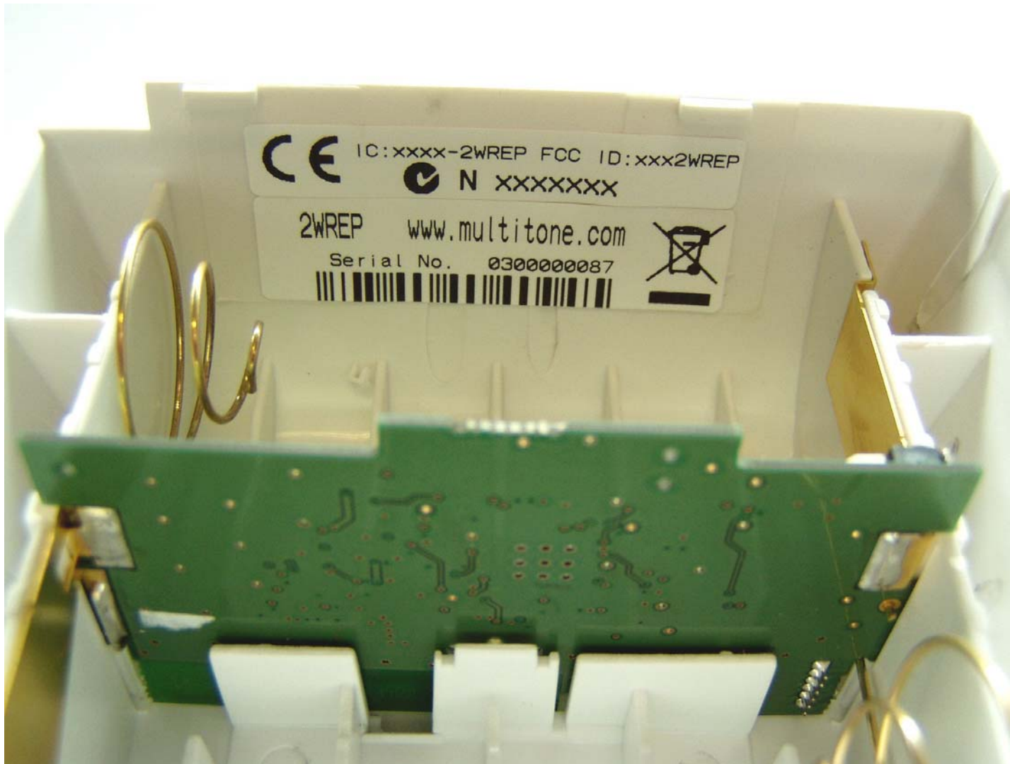
EkoTek Repeater - Label & Label Area
