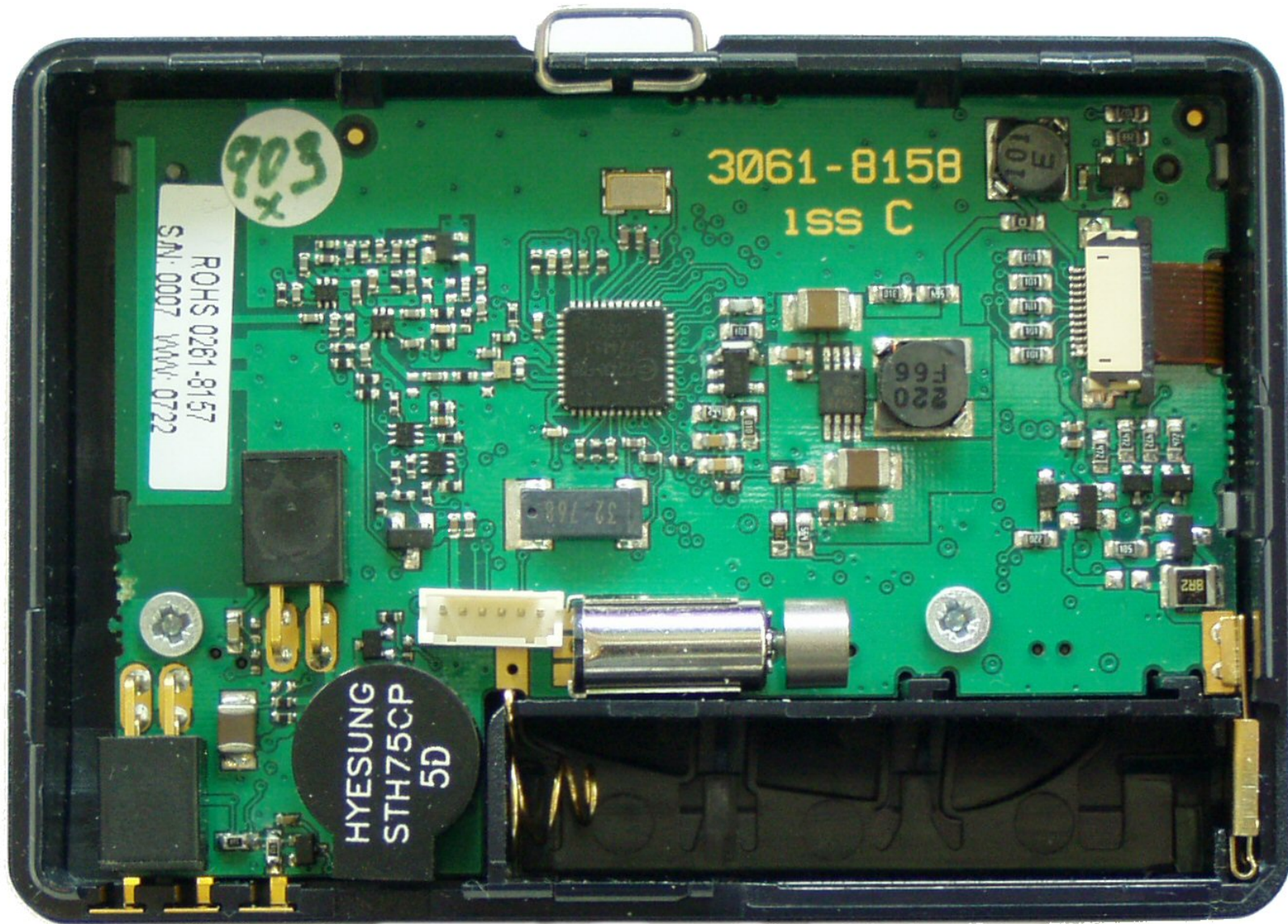
EkoTek Pager - General Internal View
