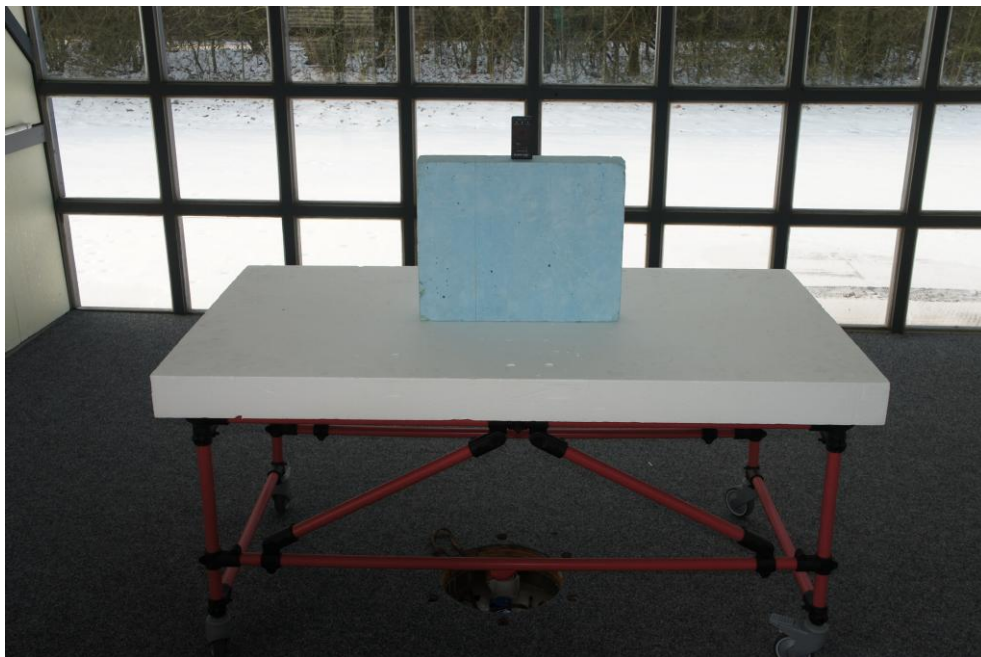
Picture 2: EUT test setup radiated emission test (30MHz to 1000MHz)
