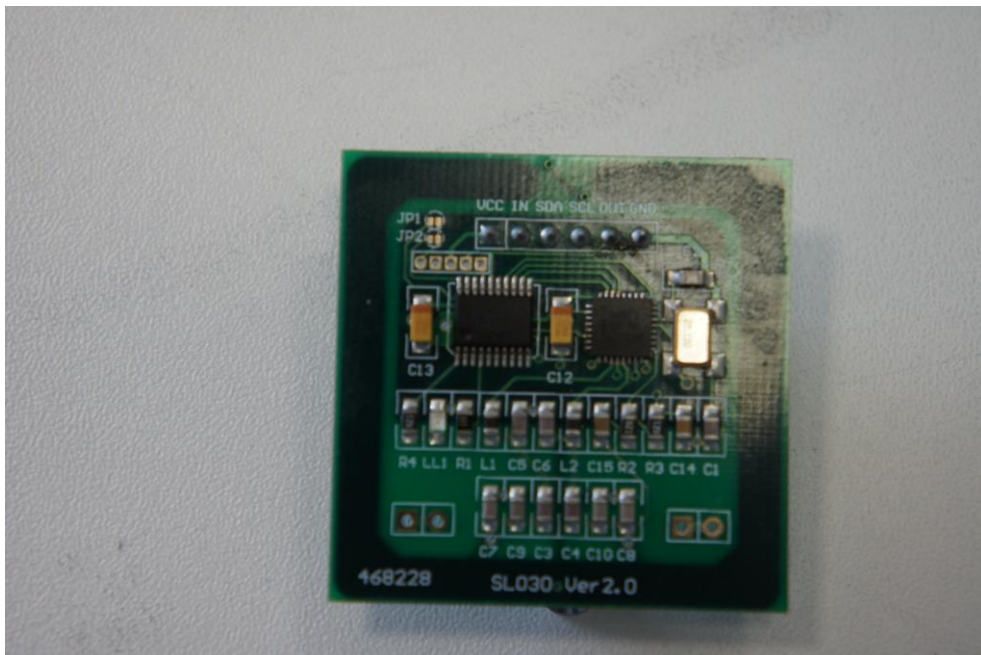
Picture 4: RFID PCB top side
