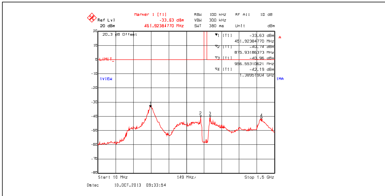
Plot 5.3.4.2.3. Conducted Spurious Emissions, High Power, 915.000 MHz, 10 MHz - 1.5 GHz
