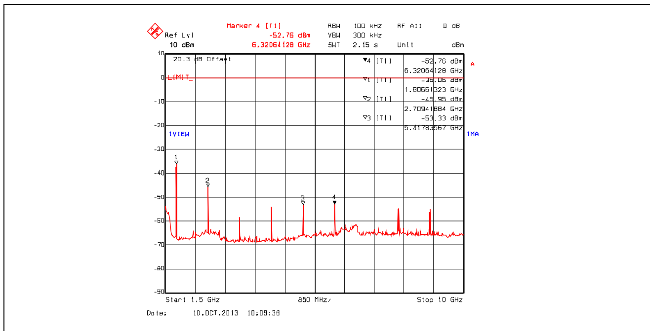
Plot 5.3.4.2.2. Conducted Spurious Emissions, High Power, 903.315 MHz, 1.5 GHz - 10 GHz
