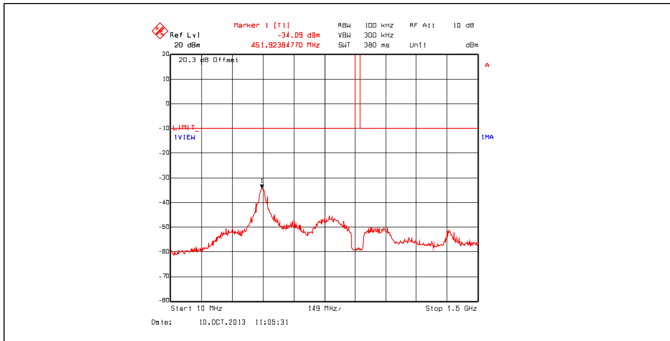
Plot 5.3.4.2.7. Conducted Spurious Emissions, Low Power, 903.315 MHz, 10 MHz - 1.5 GHz
