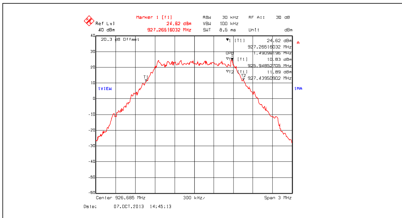
Plot 5.1.4.6. 99% Occupied Bandwidth, 926.685 MHz
