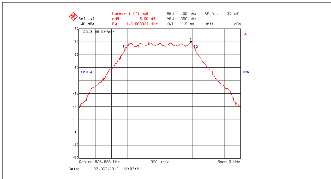
Plot 5.1.4.3. 6 dB Bandwidth, 926.685 MHz
