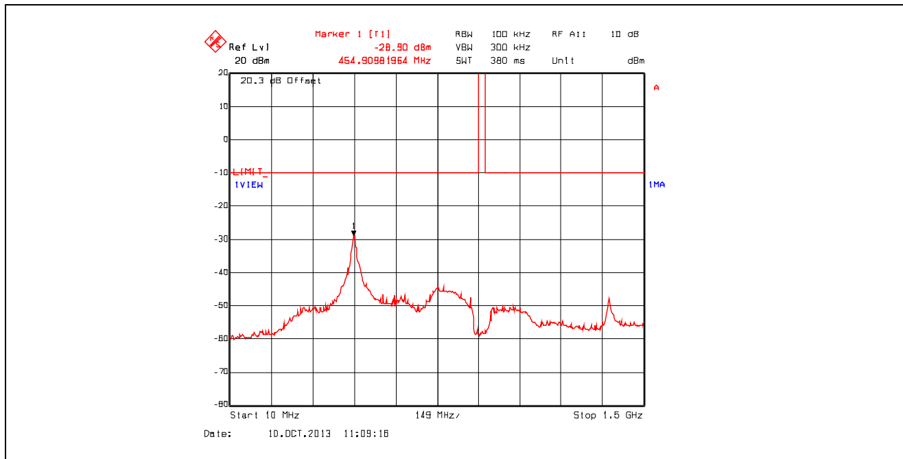
Plot 5.3.4.2.9. Conducted Spurious Emissions, Low Power, 915.000 MHz, 10 MHz - 1.5 GHz
