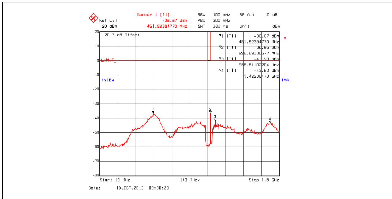
Plot 5.3.4.2.5. Conducted Spurious Emissions, High Power, 926.685 MHz, 10 MHz - 1.5 GHz
