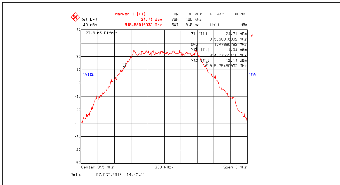
Plot 5.1.4.5. 99% Occupied Bandwidth, 915.000 MHz
