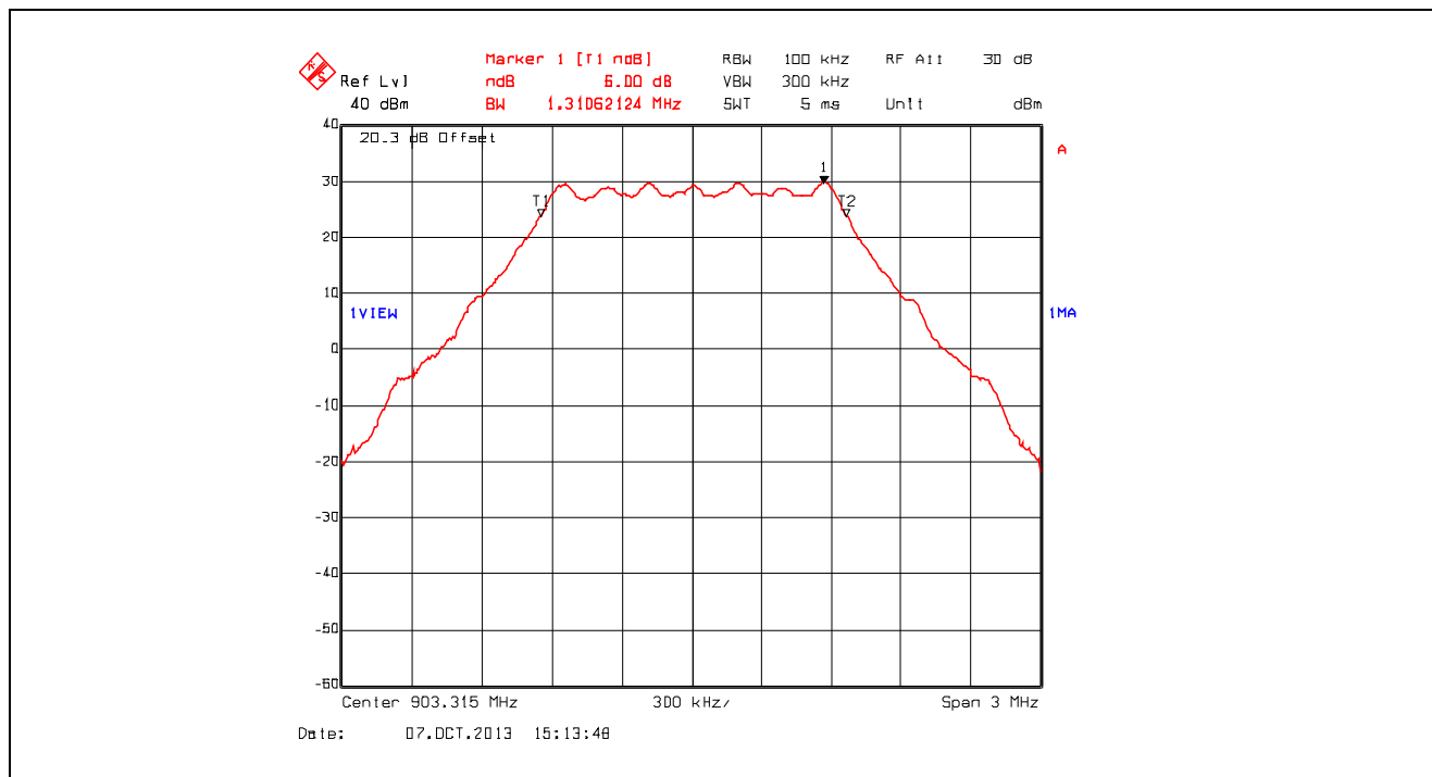
Plot 5.1.4.1. 6 dB Bandwidth, 903.315 MHz
