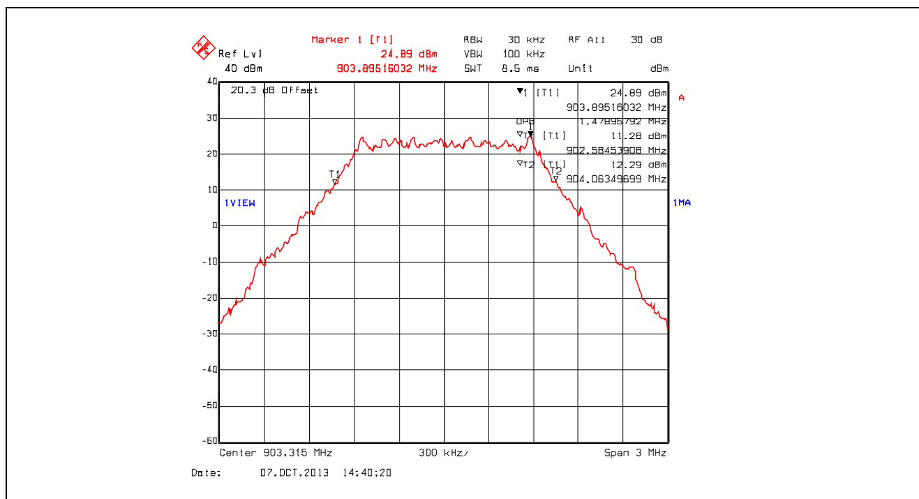
Plot 5.1.4.4. 99% Occupied Bandwidth, 903.315 MHz
