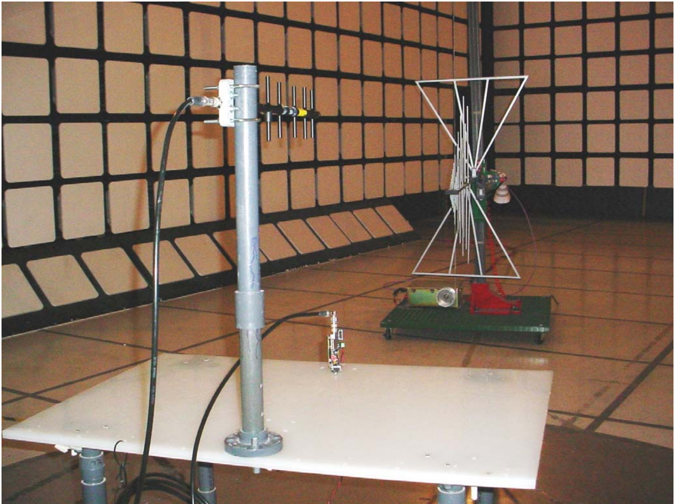
Radiated Emission Setup (Yagi Antenna)
