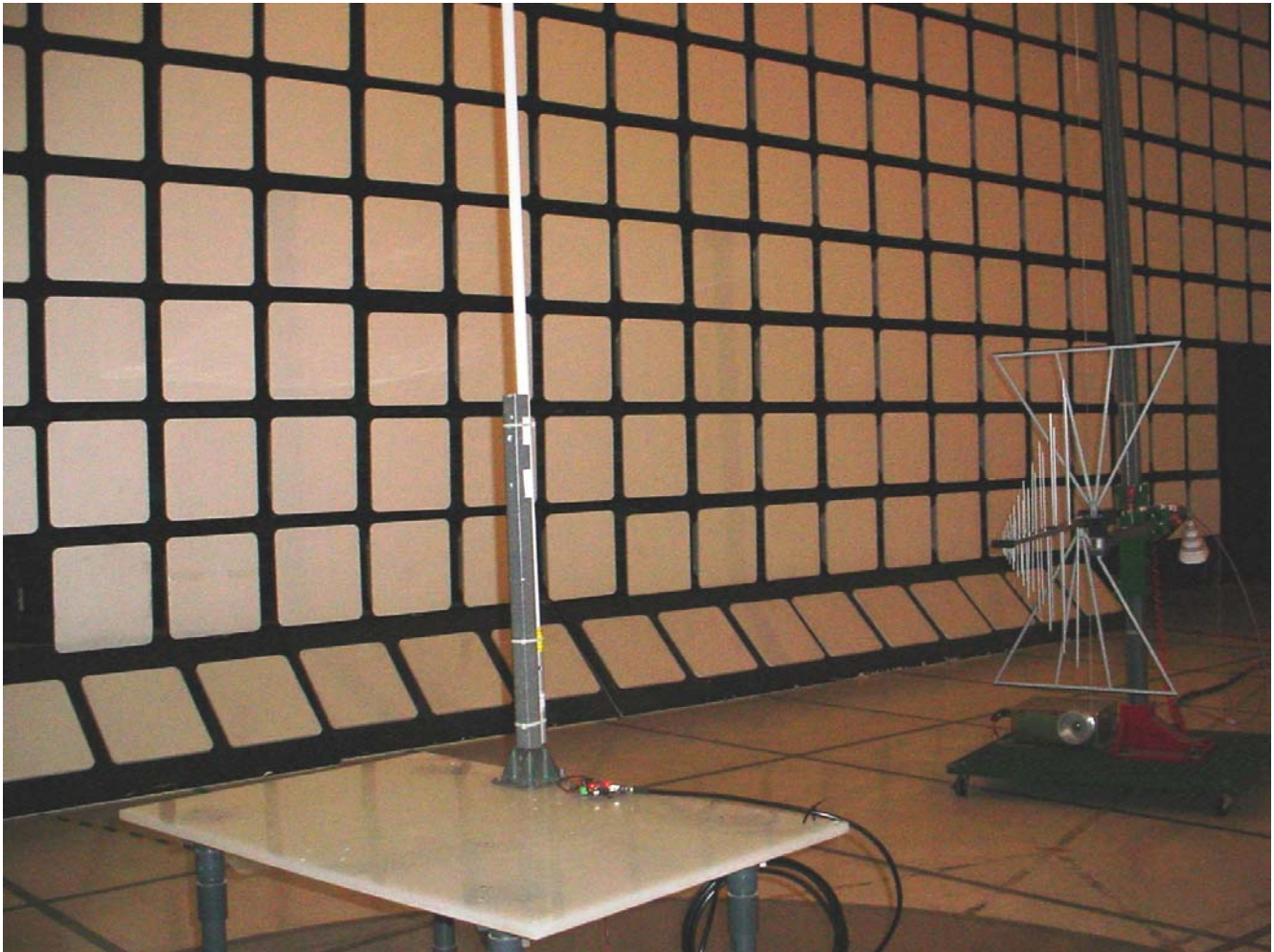
Radiated Emission Setup (Omni Antenna)
