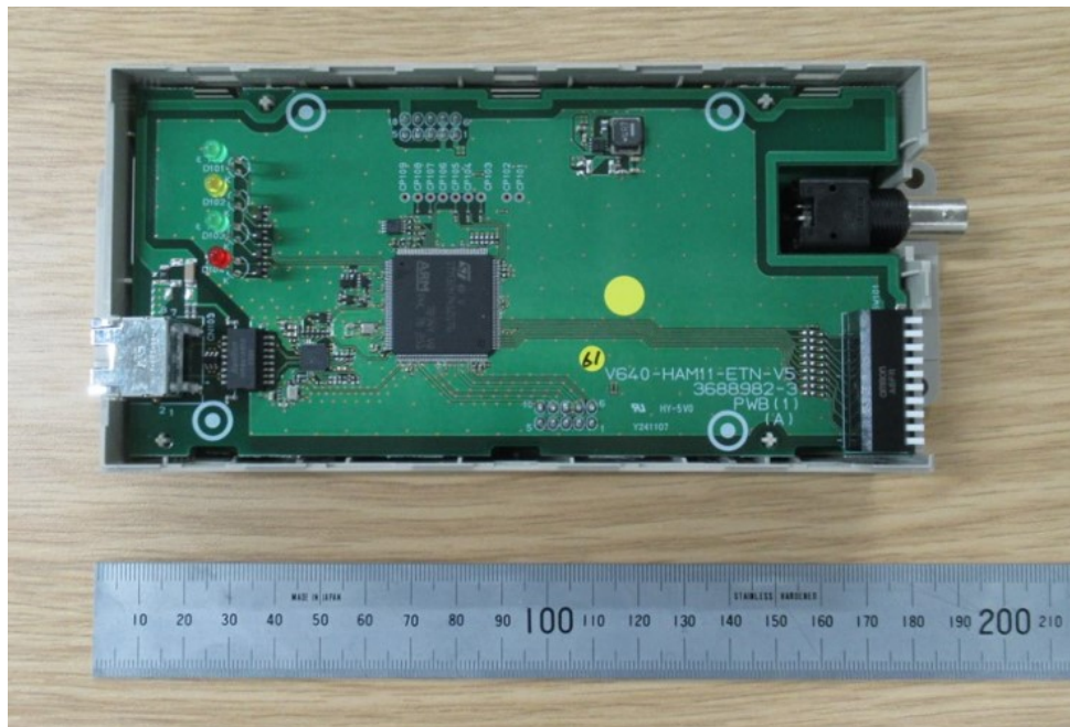
PCB(1) – Side A (74.0 x 154.5 mm)
