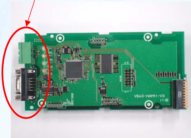
Inside of V640-HAM11-L
