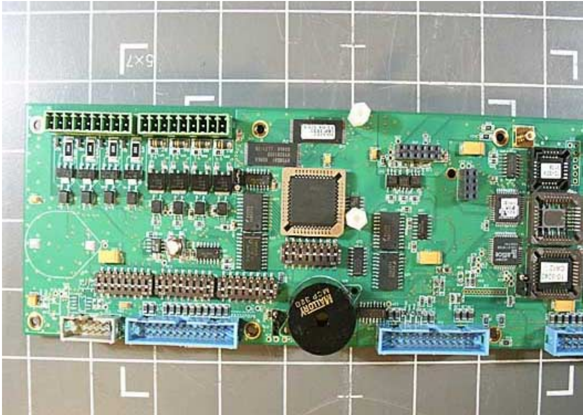
Front PCB Top Left
