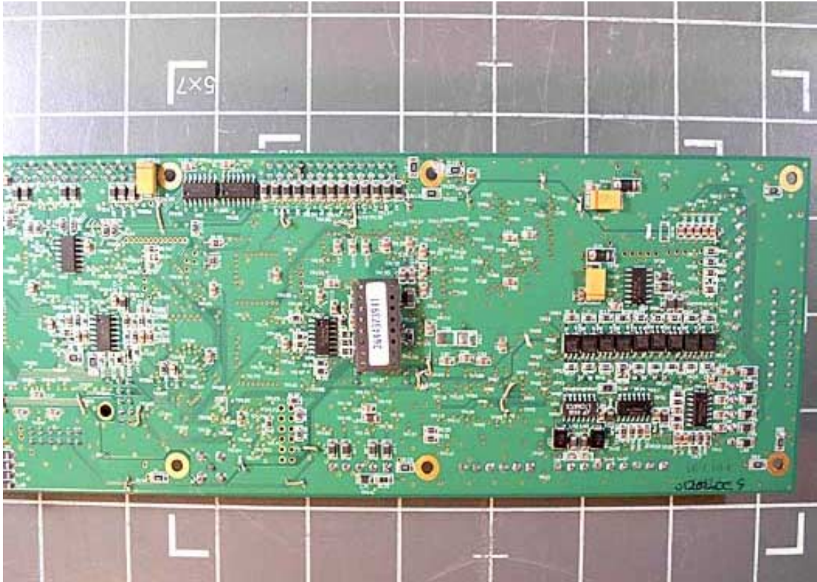
Front PCB Bottom Right
