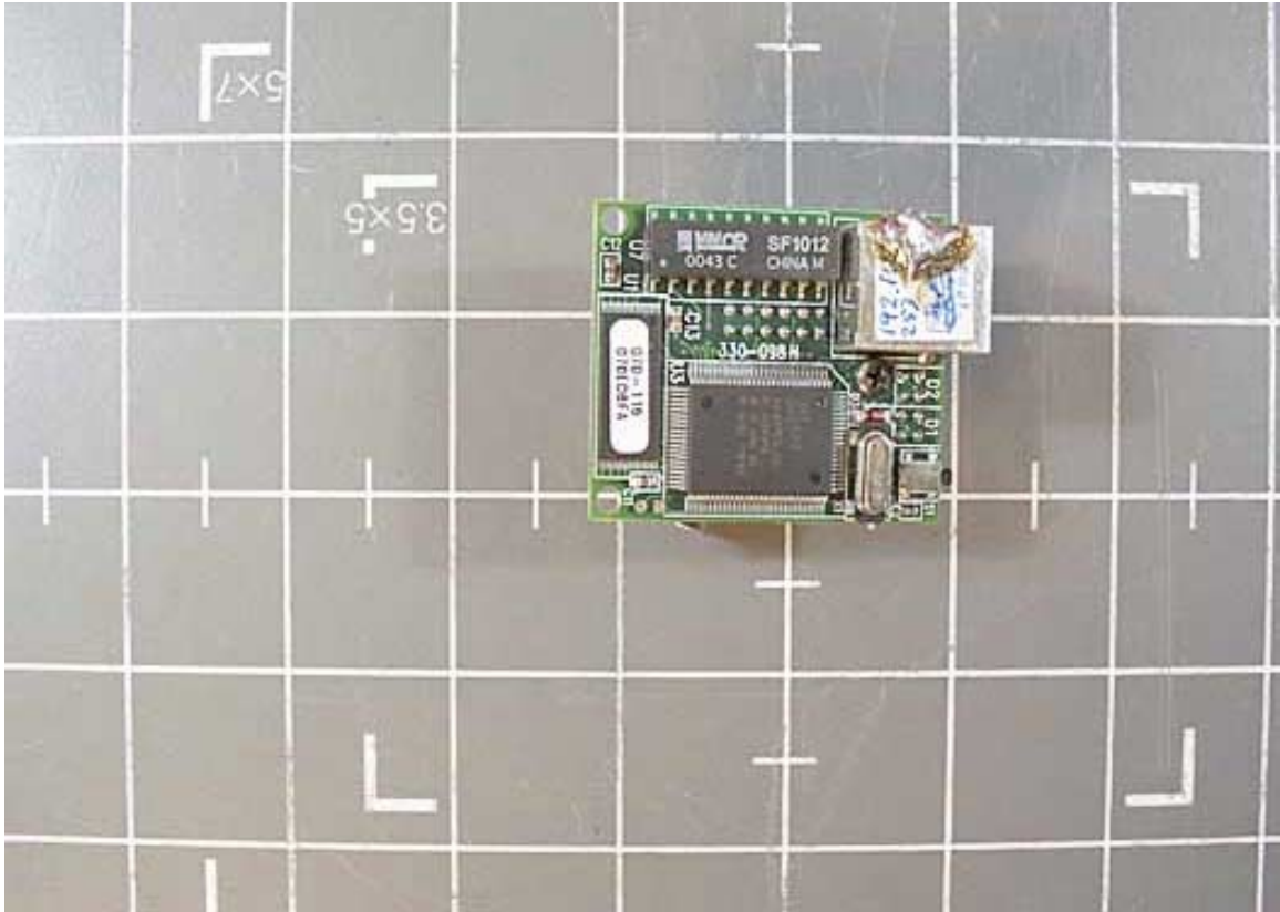
Daughter PCB Top
