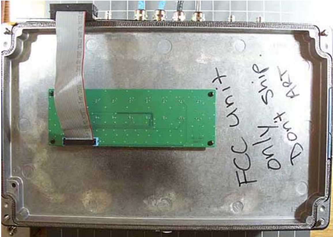
Inside Top Lid – LED PCB Back
