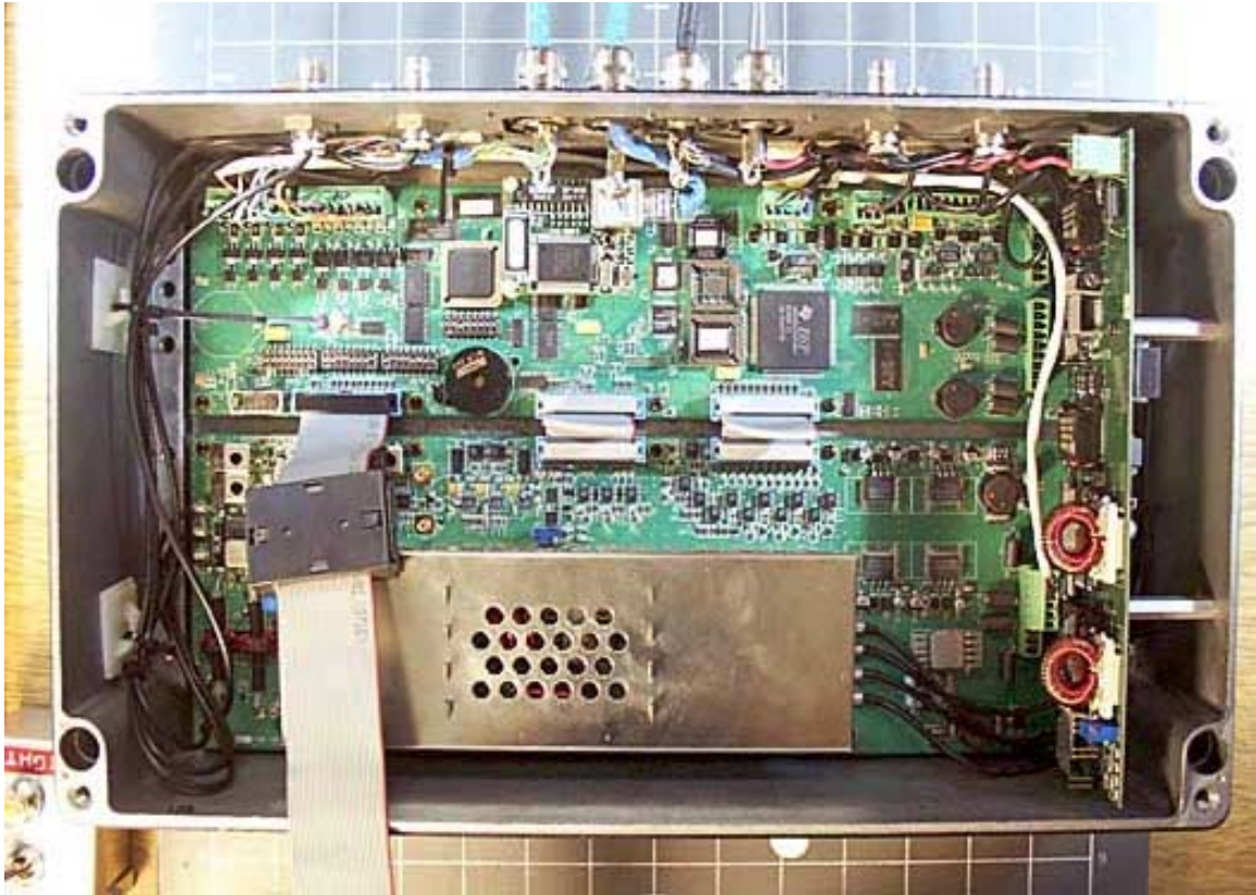
Inside Chassis Layout
