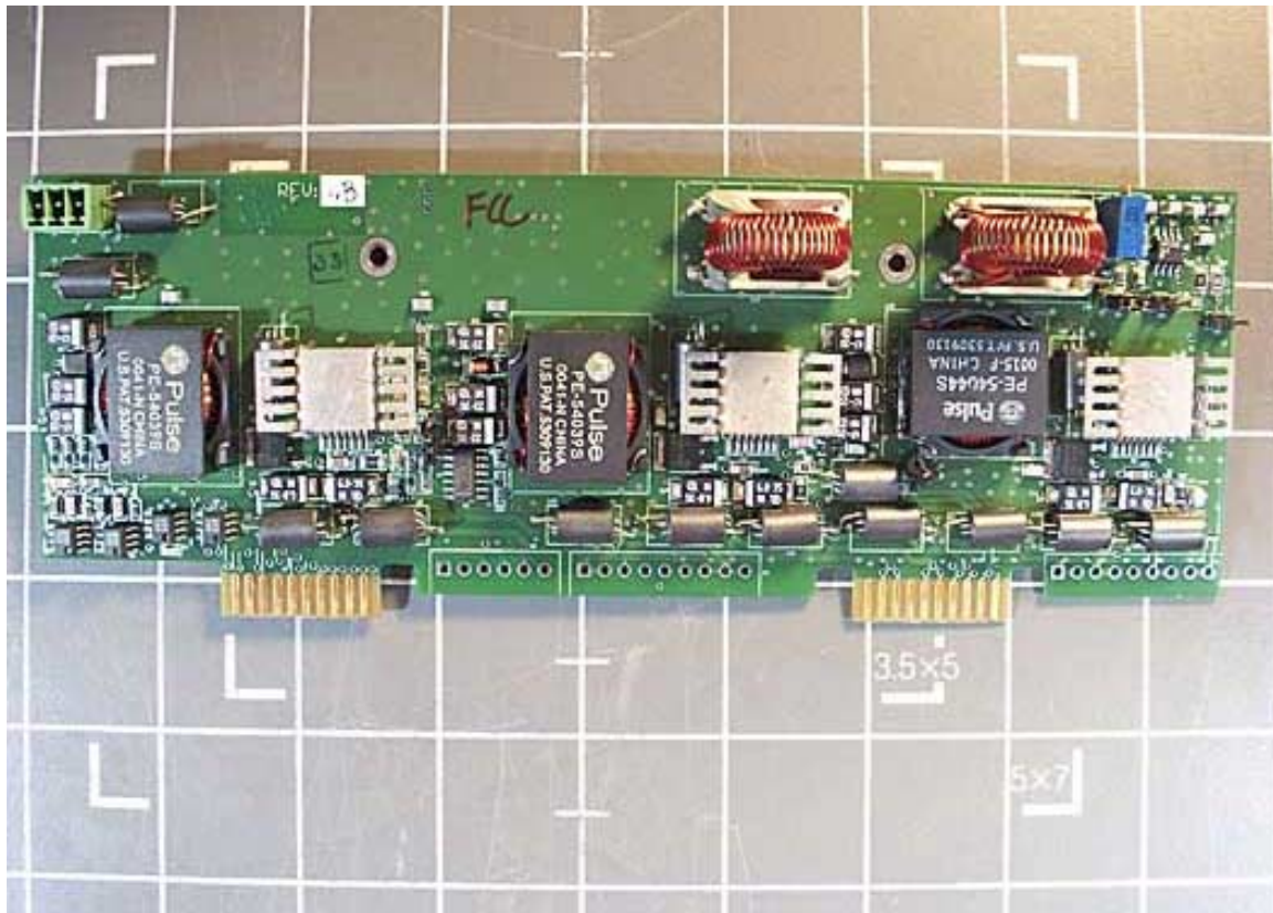
Riser PCB Component Side
