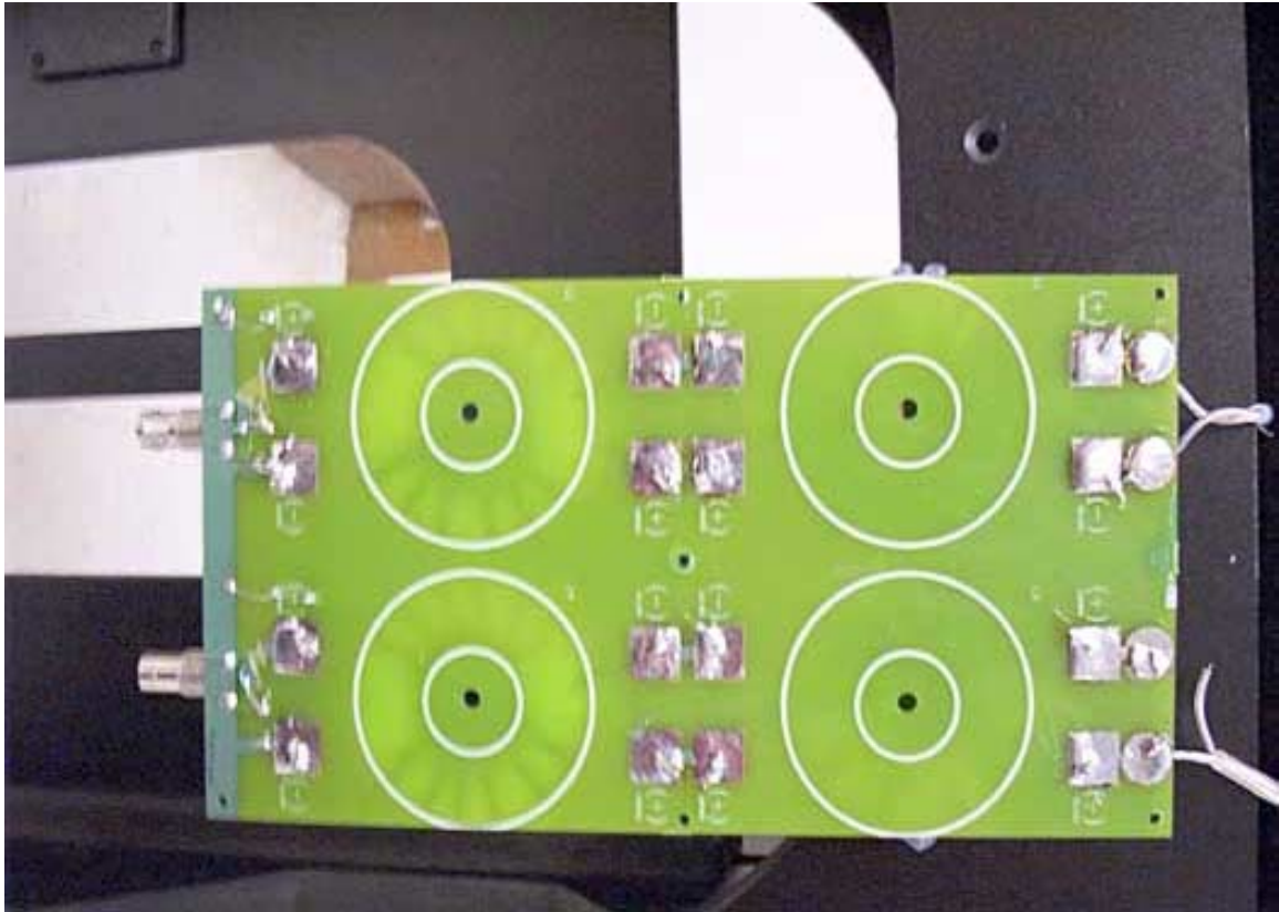
Antenna PCB Back Side
