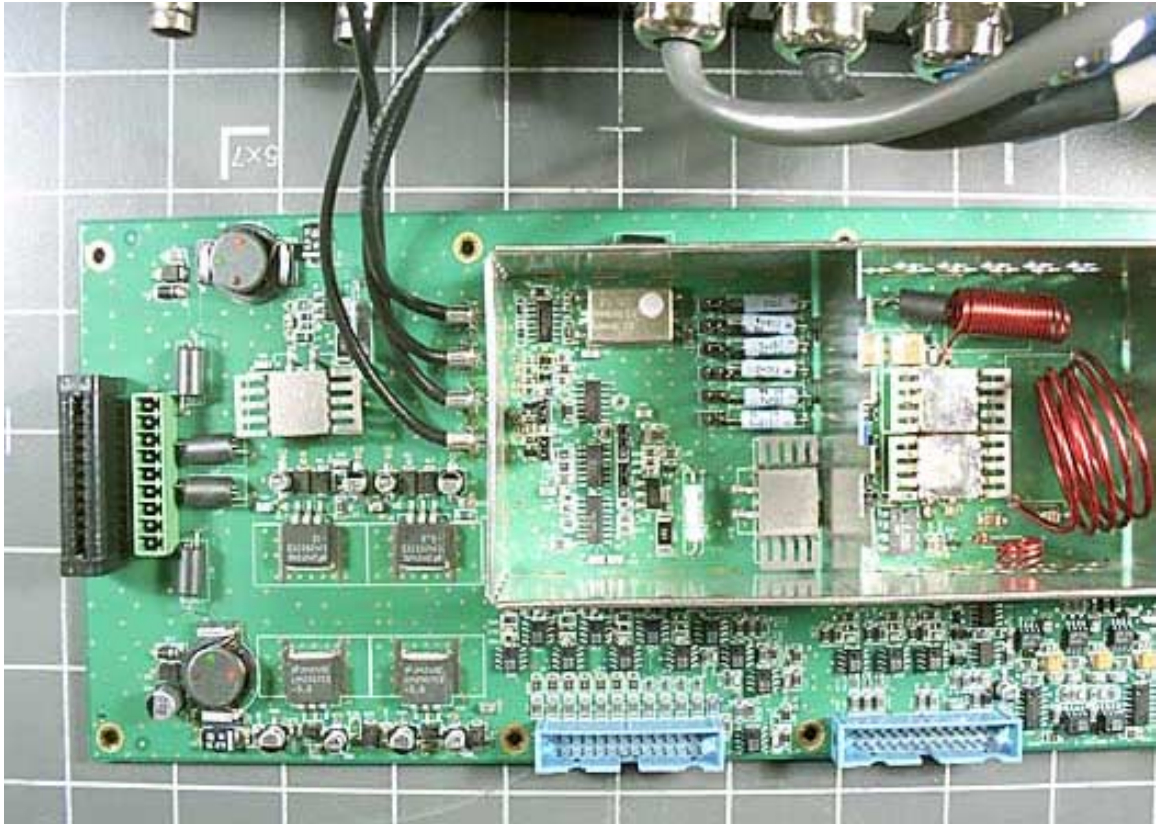
Rear PCB Top Left
