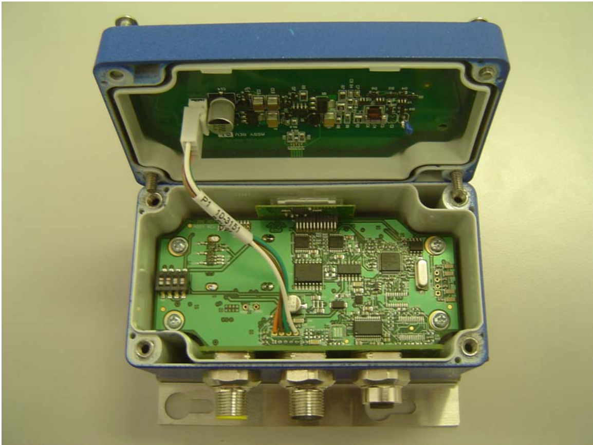
CHS1265 Front/Top View (Opened)
