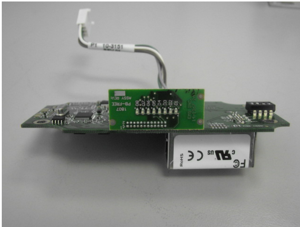
CHS1265 Main PCB Assembly Front View (w/ LED Module PCB)
