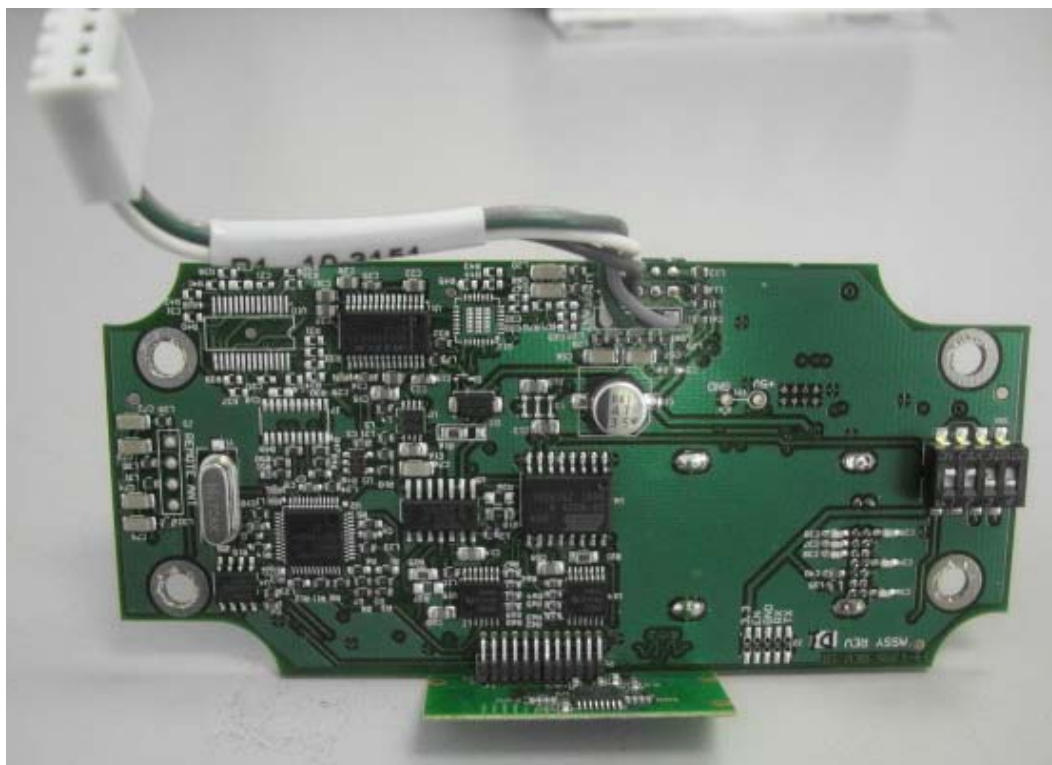
CHS1265 Main PCB Assembly Top View
