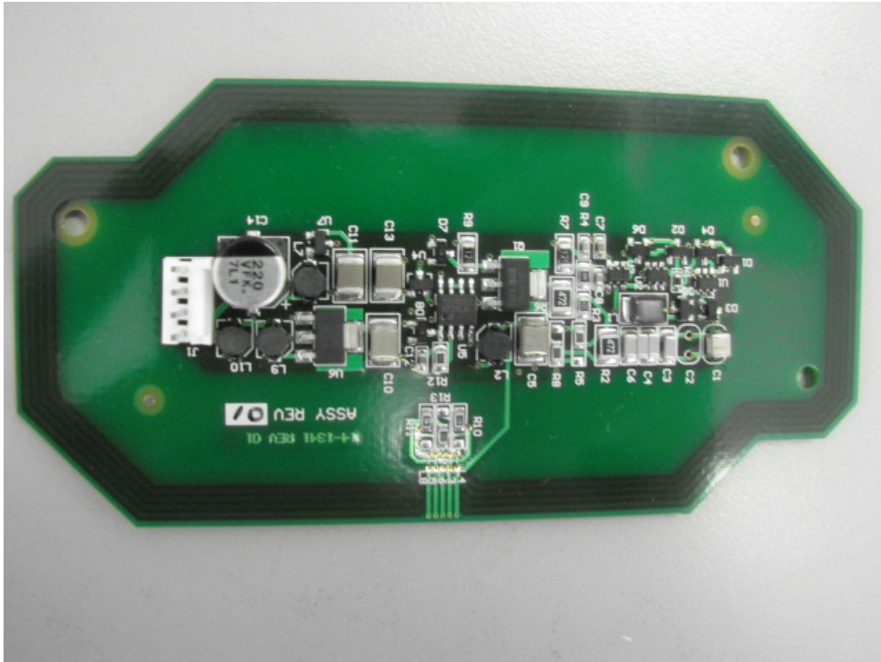
CHS1265 Main PCB Assembly Bottom View
