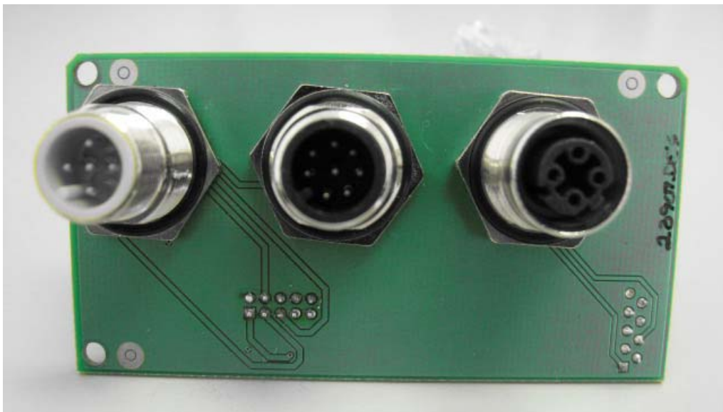
CHS1265 Connector PCB Assembly Front View
