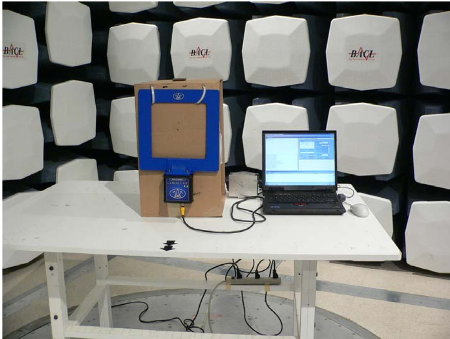
Radiated Emission Greater than 30MHz – Front View
