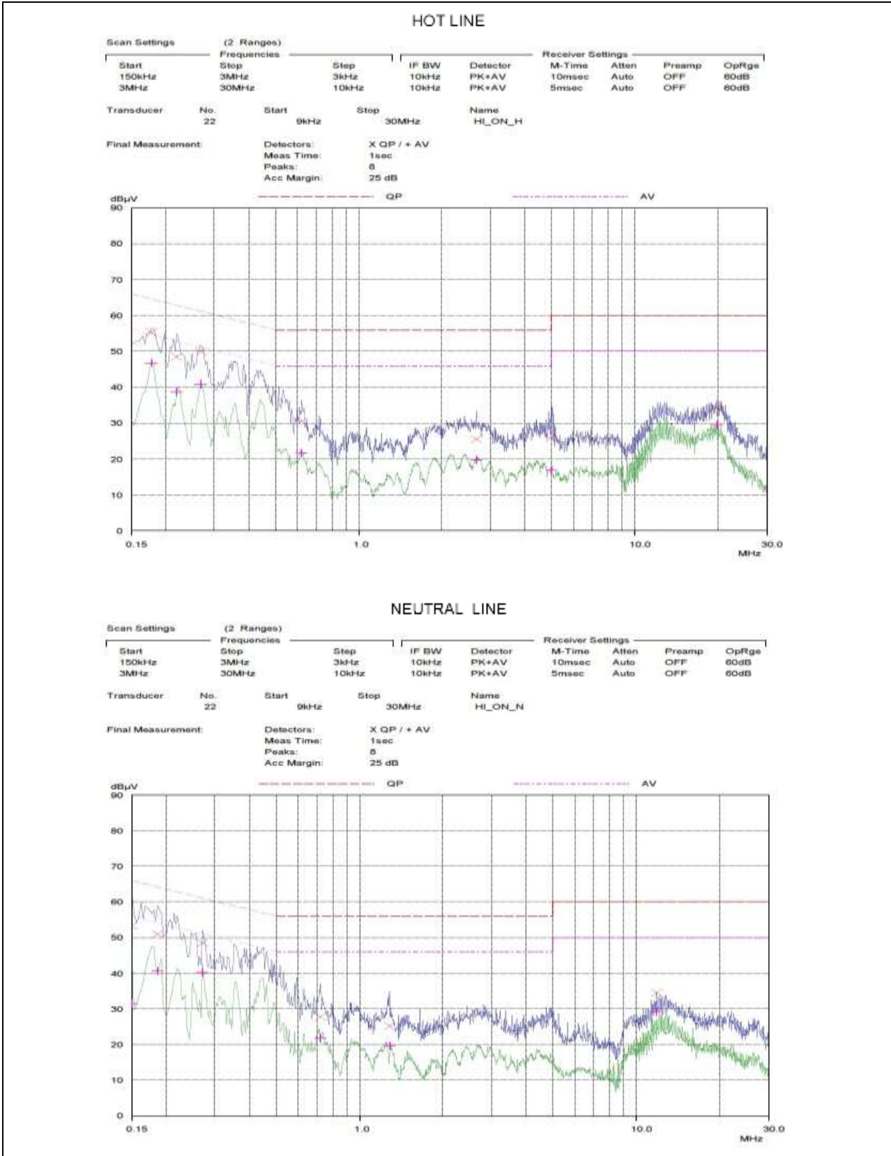
Figure 6. Graphical representation of Conducted Emission
