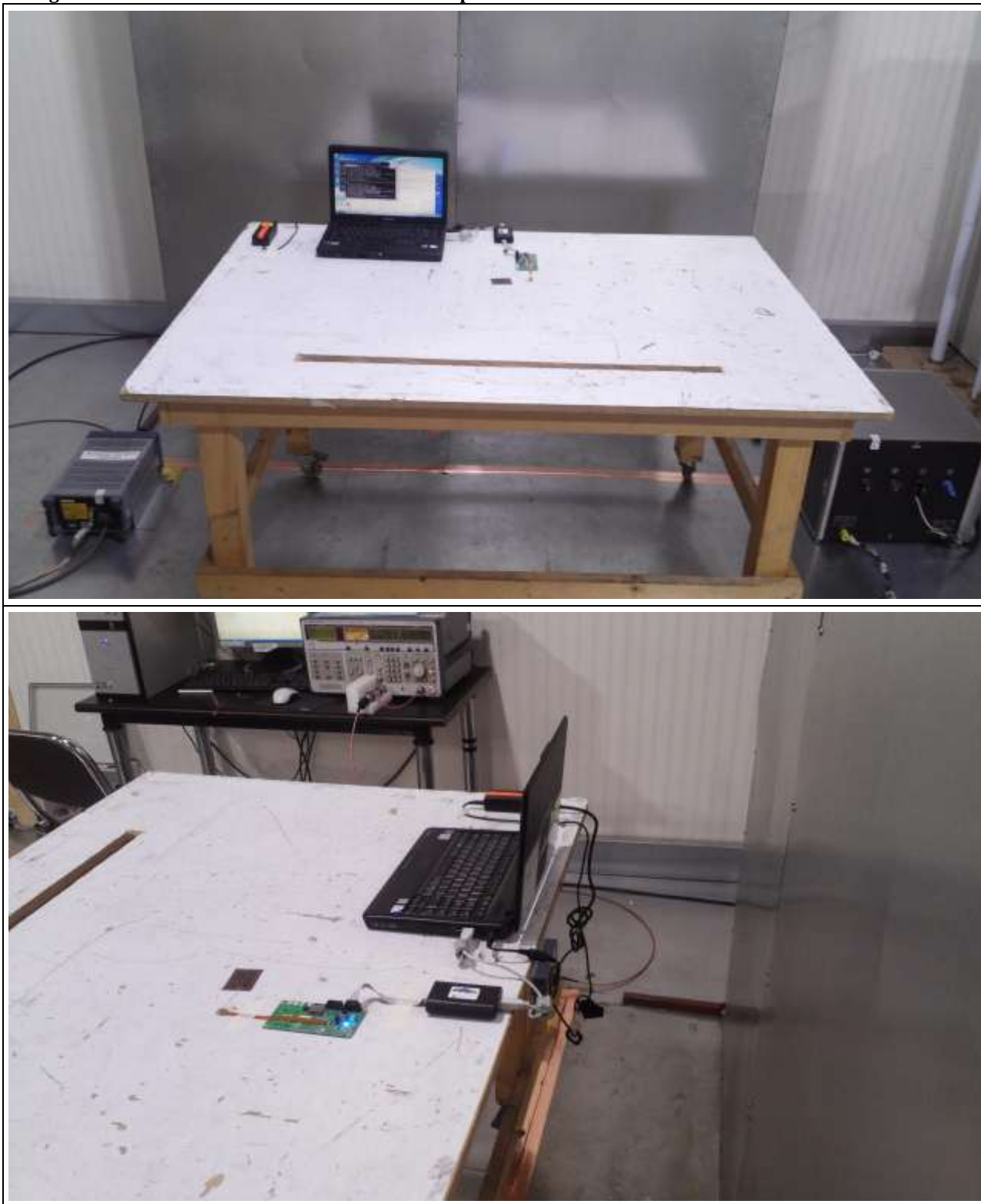
Figure 2. Photo of Conducted Emission Test Setup
