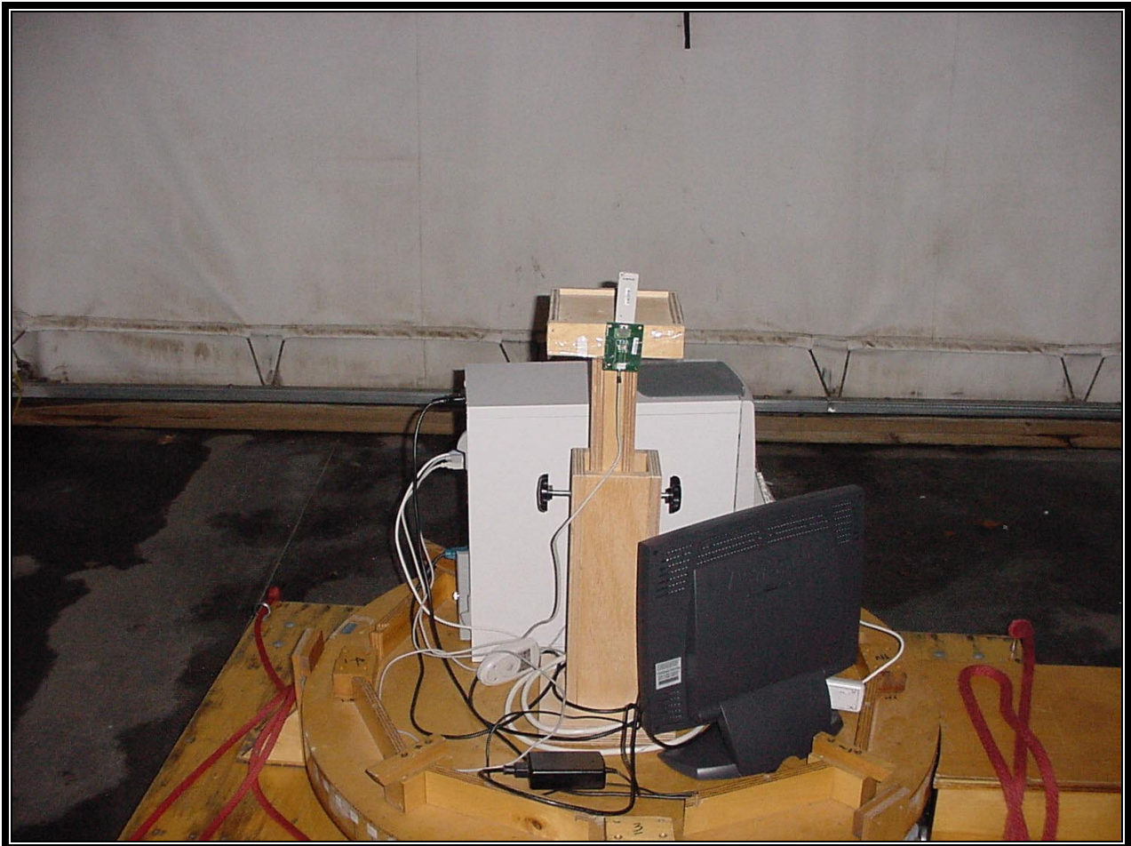
PHOTOGRAPH 3: RADIATED EMISSIONS REAR VIEW WORST CASE CONFIGURATION
