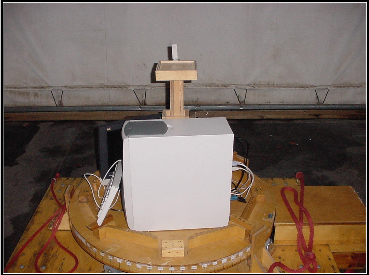
PHOTOGRAPH 2: RADIATED EMISSIONS FRONT VIEW WORST CASE CONFIGURATION
