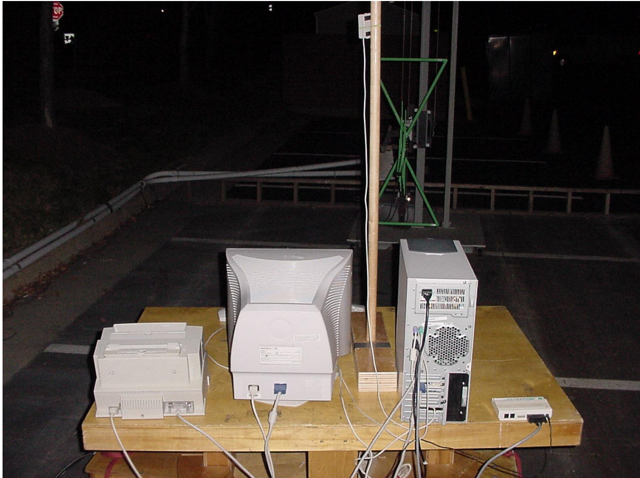
PHOTOGRAPH 4: RADIATED EMISSION REAR VIEW CASE CONFIGURATION
