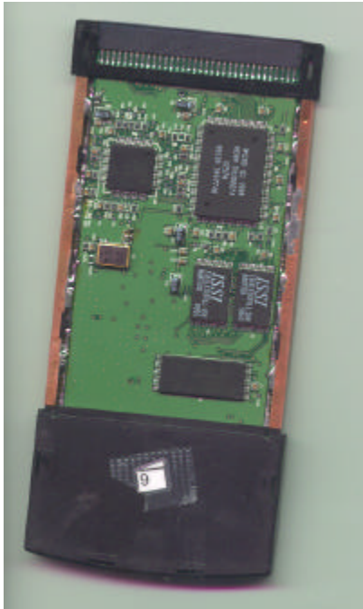
Figure 5: PCM Solder Side
