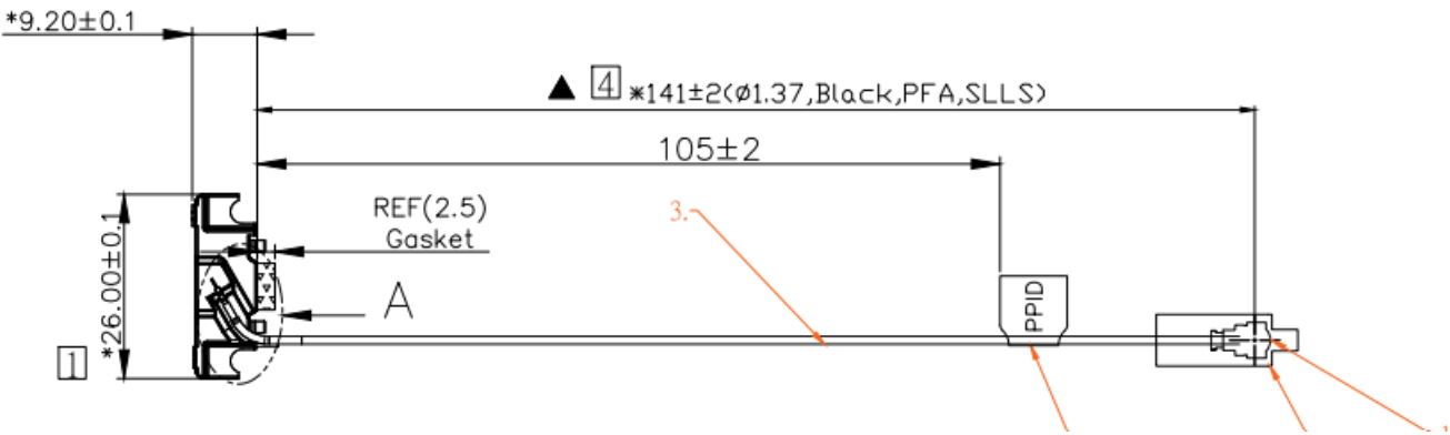
Aux Antenna Drawing:
