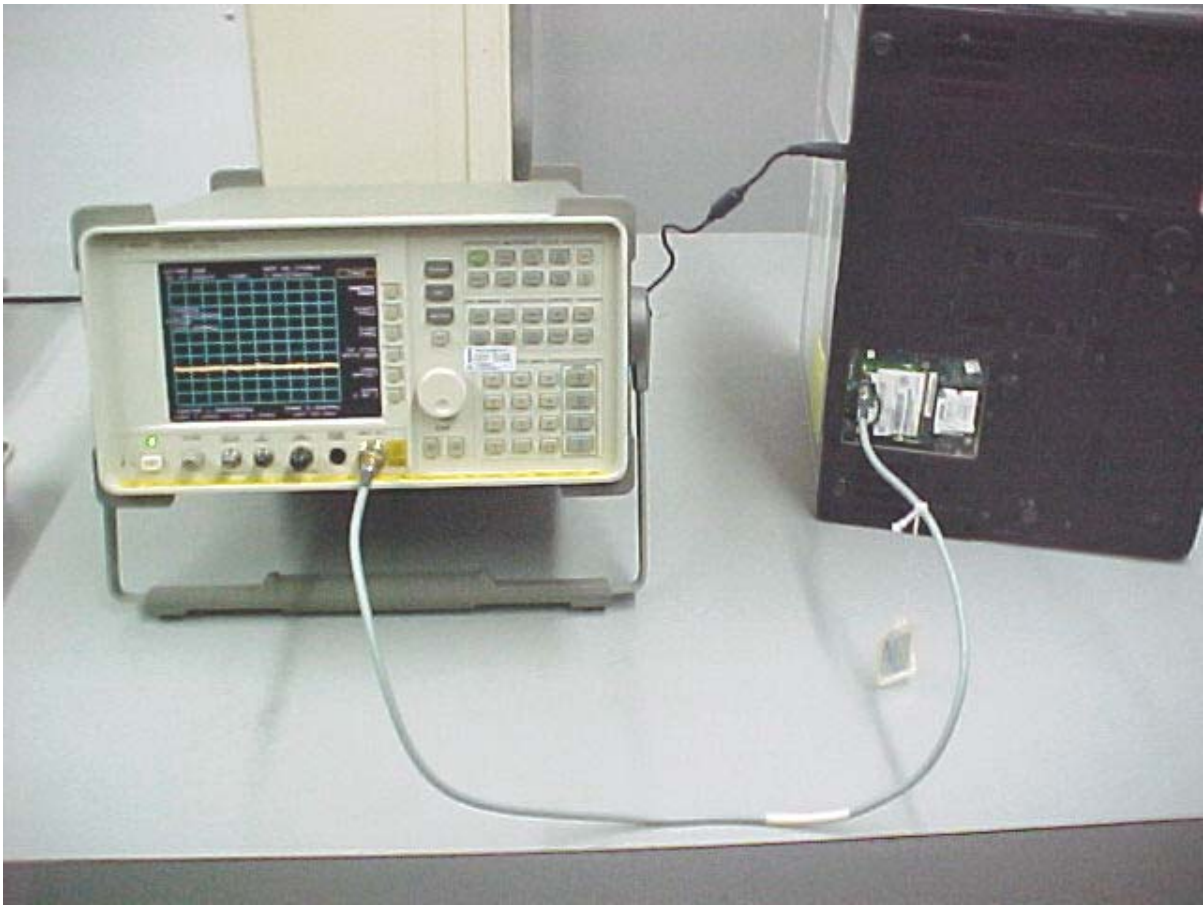
Conducted Emissions at Antenna Terminal Setup
