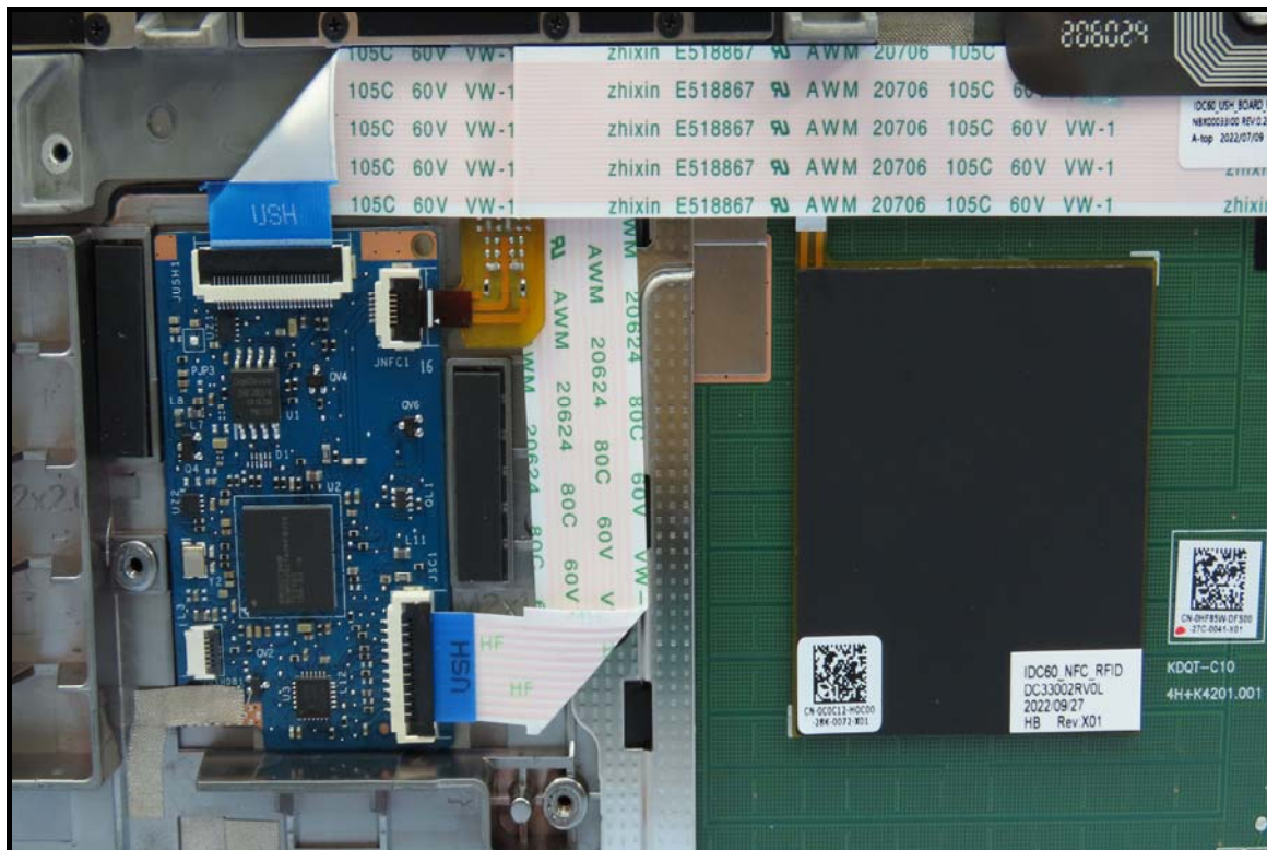
Hong-Bo antenna
