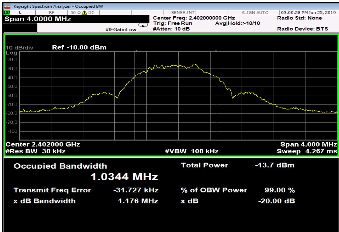
Occupied Bandwidth – Low Channel
