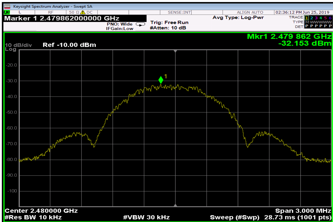
Peak PSD – High Channel
