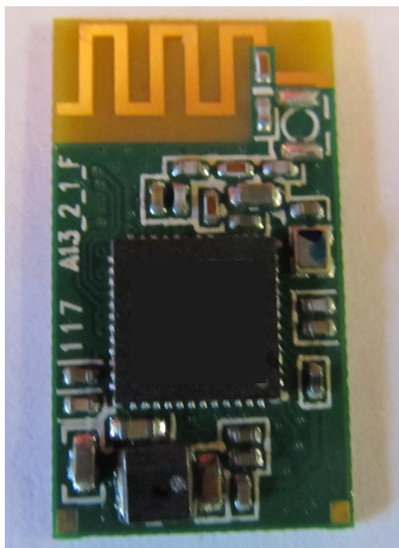
Top Side - Internal
