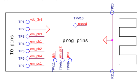
Approximate pin positions on board layout
