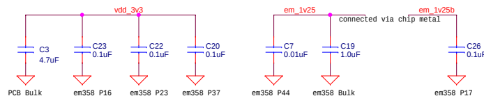
Bypass Caps
