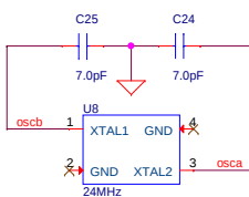
XTAL shield intentionally left floating
