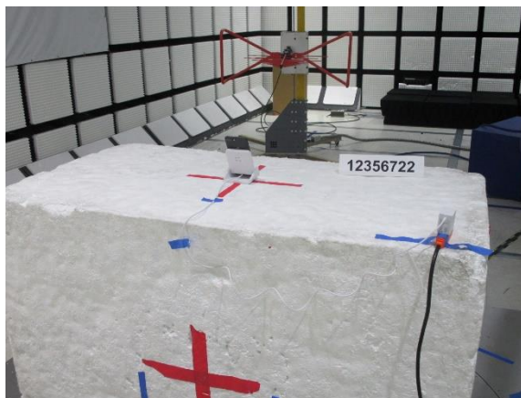
Operating Mode With Phone Back
