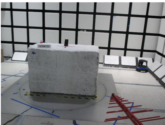
Operating Mode With Phone Front
