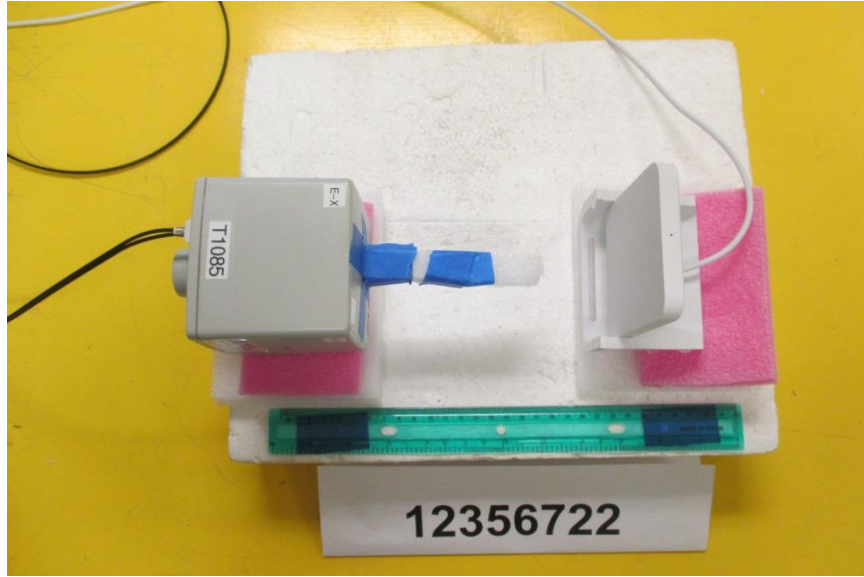
CENTER, RF EXPOSURE SETUP PHOTO
