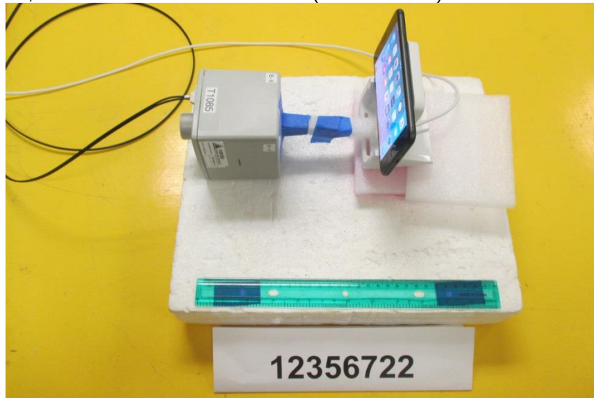
S4, RF EXPOSURE SETUP PHOTO (HORIZONTAL)
