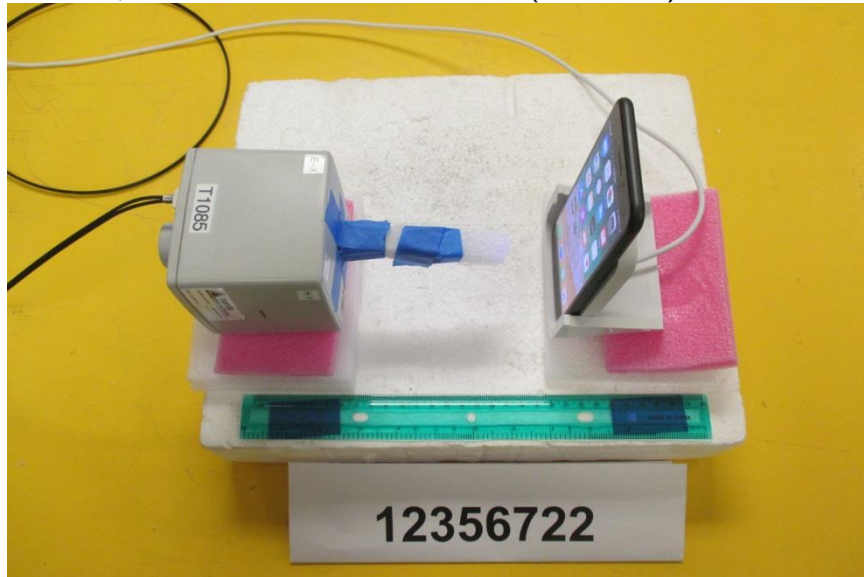
CENTER, RF EXPOSURE SETUP PHOTO (VERTICAL)
