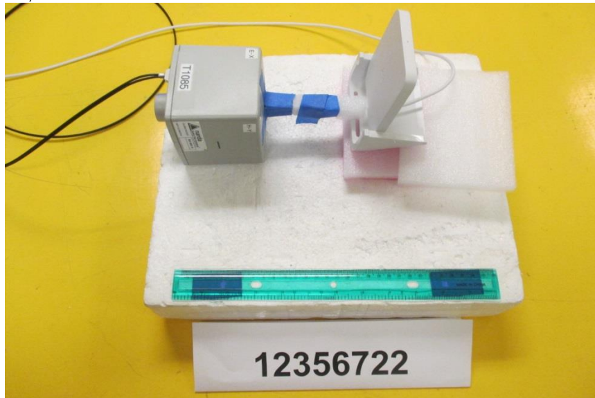
S4, RF EXPOSURE SETUP PHOTO
