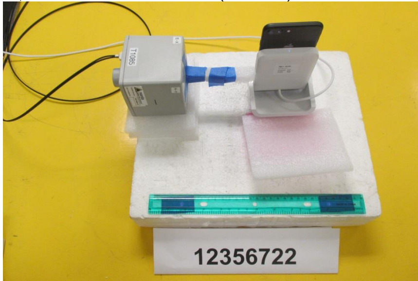
S3, RF EXPOSURE SETUP PHOTO (VERTICAL)
