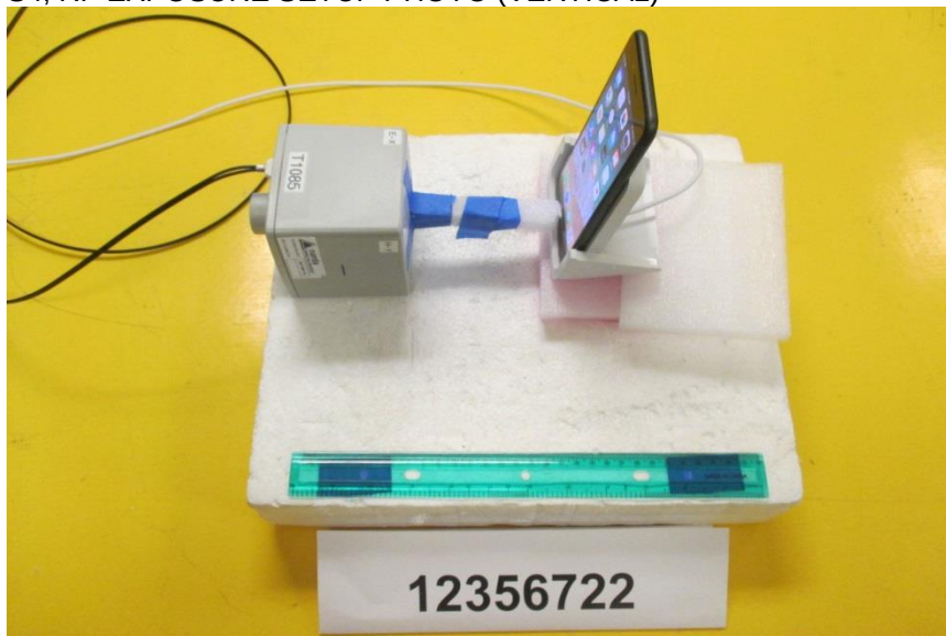
S4, RF EXPOSURE SETUP PHOTO (VERTICAL)
