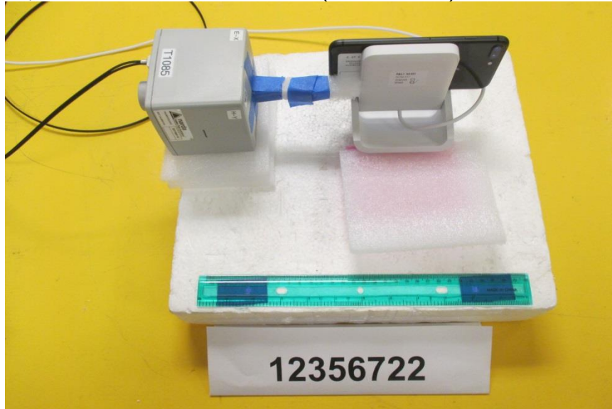
S3, RF EXPOSURE SETUP PHOTO (HORIZONTAL)
