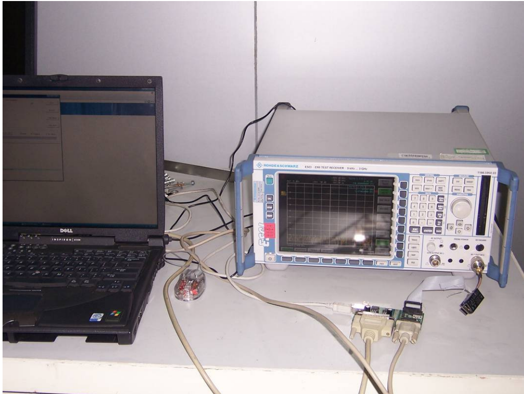
Photograph 4: Set-up for Spurious Emissions (9kHz-30MHz)
