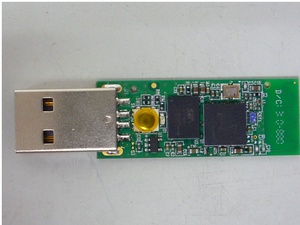
Fig. 2: Internal view
