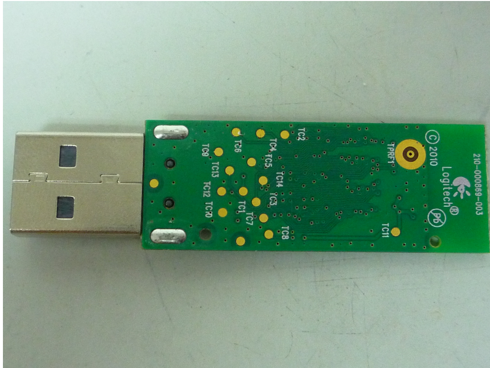
Fig. 1: Internal view
