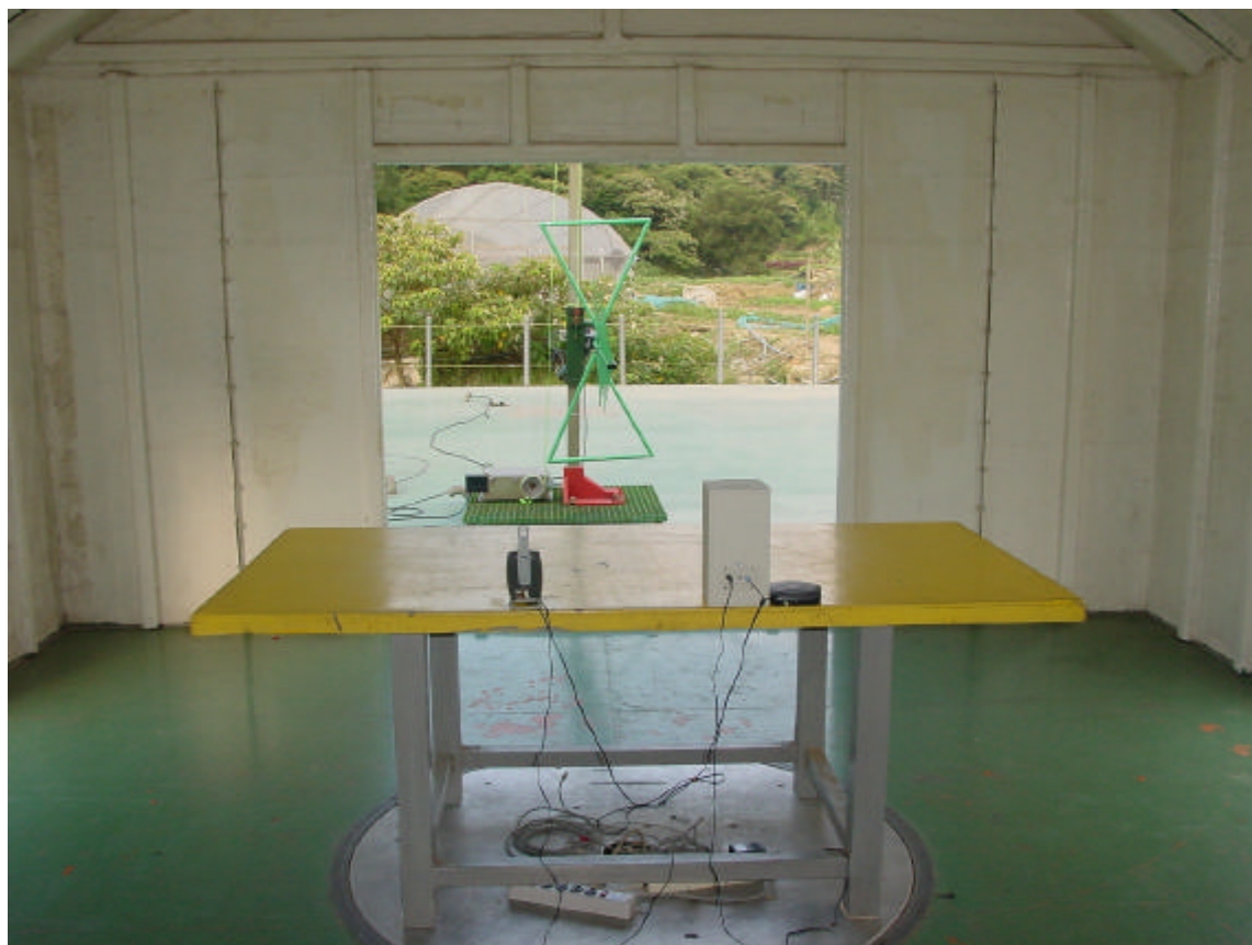
Radiated (30~1000MHz)
