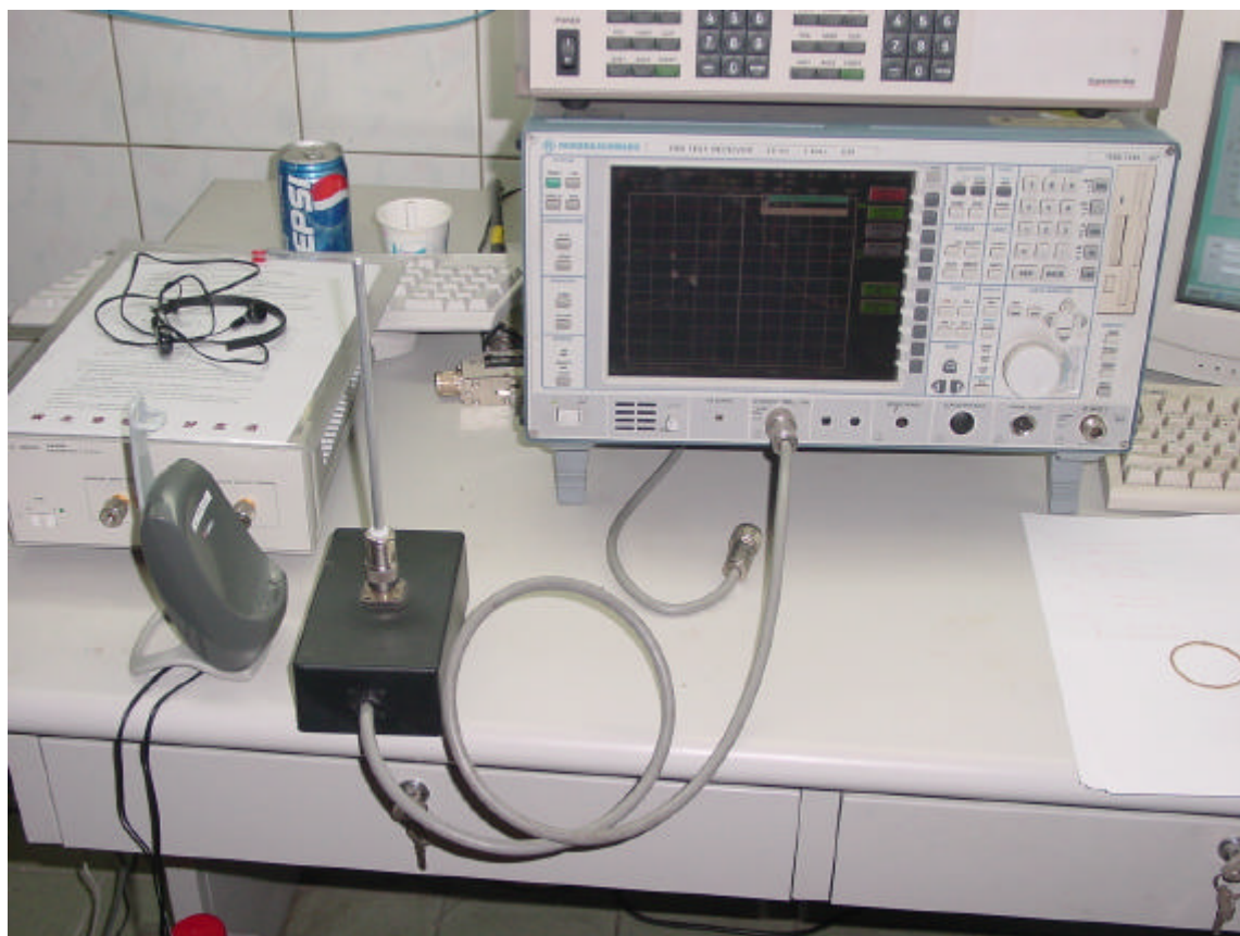
Occupied Bandwidth
