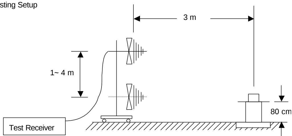
Configuration of EUT Setup
