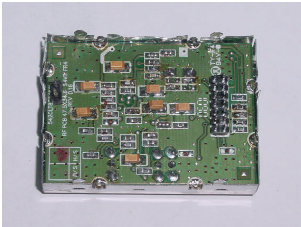
RF Module (Side 1)
