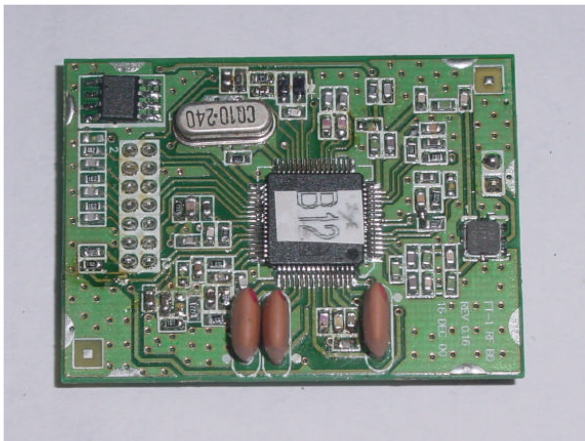
RF Module (Side 2)
