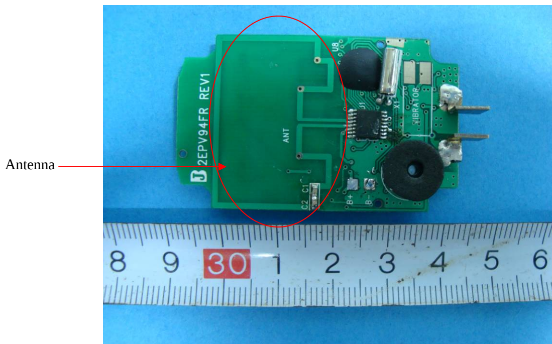
EUT- Main Board Top Component View
