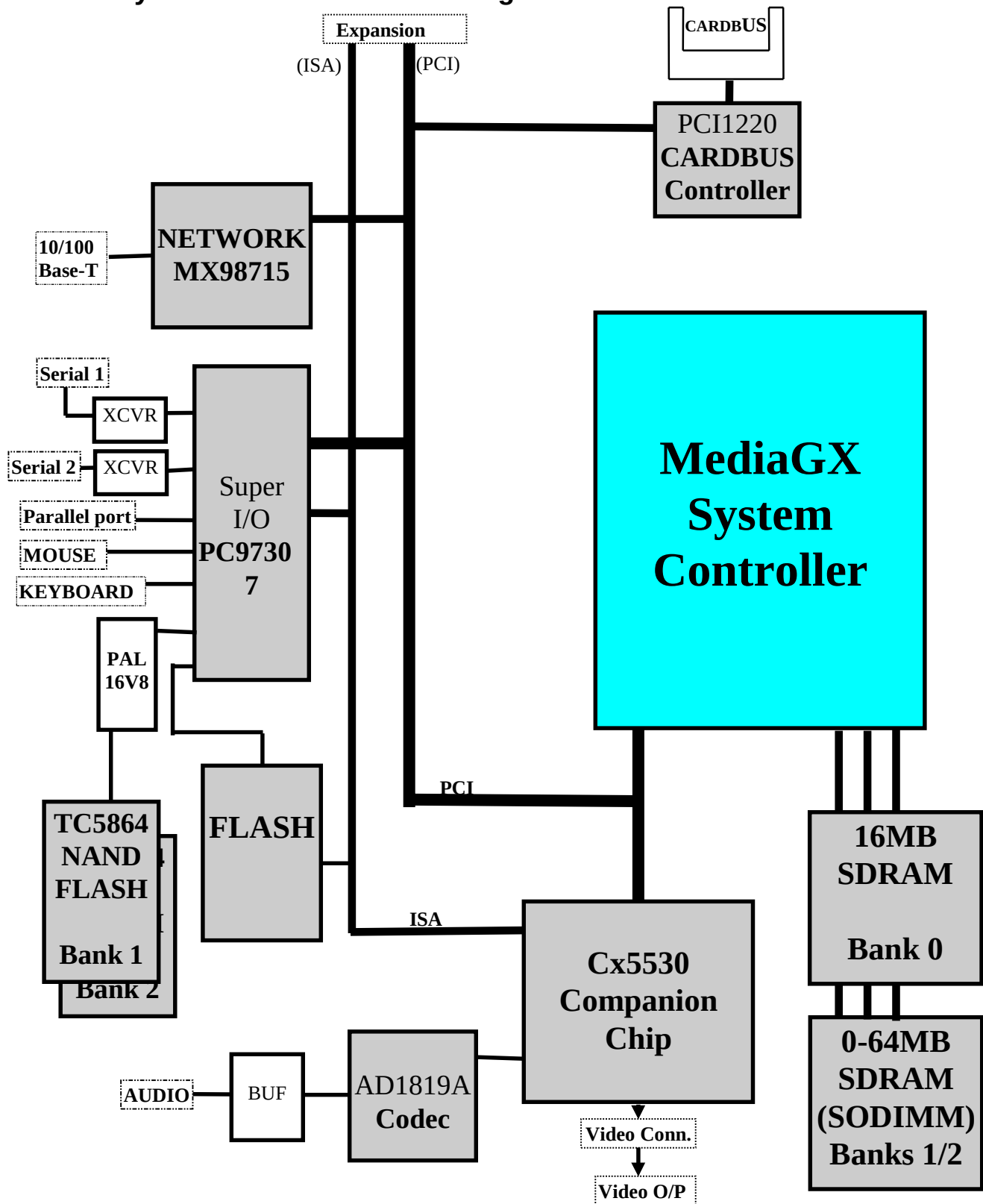
System Functional Block Diagram:
