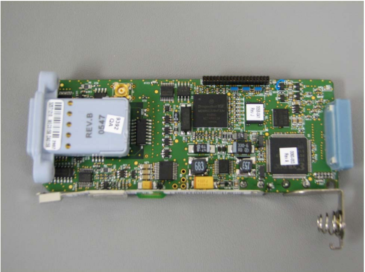
Figure 1: Baseboard Front
