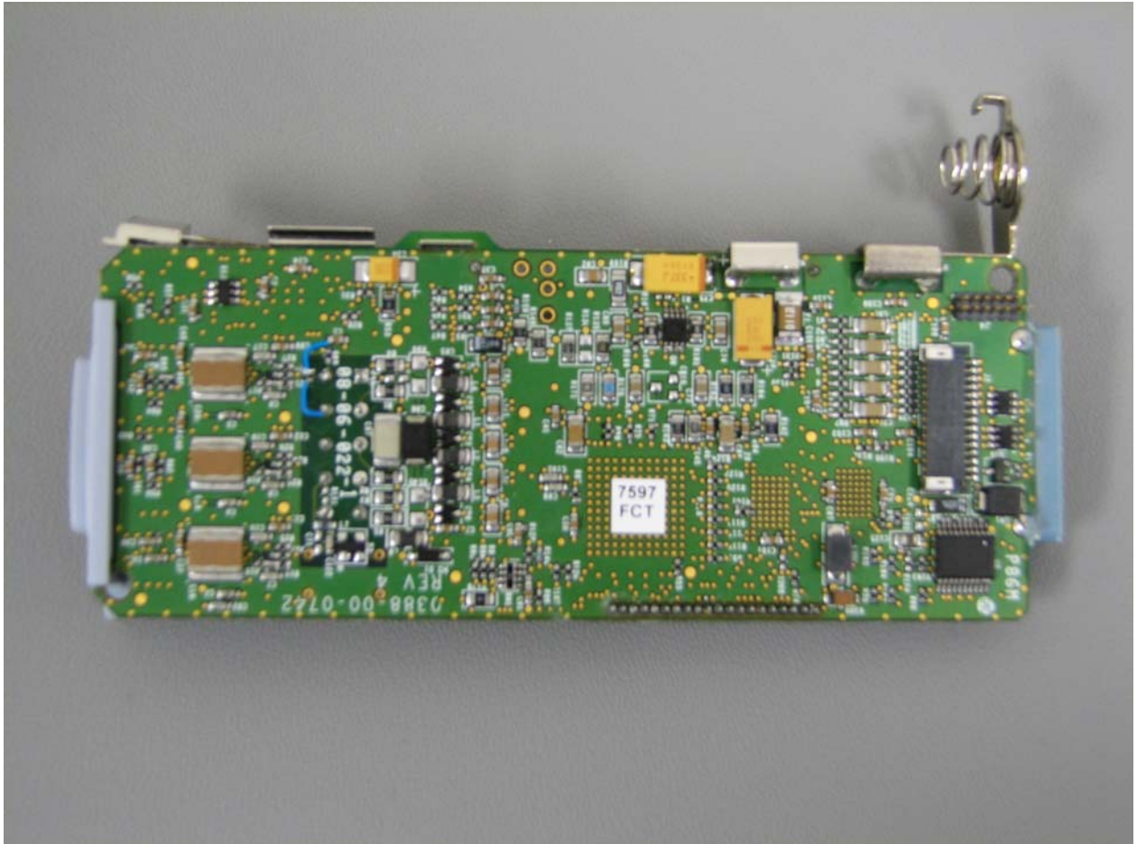
Figure 2: Baseboard Back
