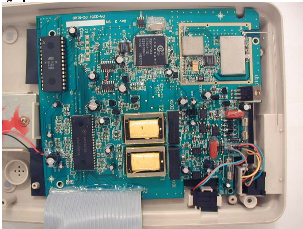
Figure 1: Base Unit – Top View - with RF Circuit Covers
