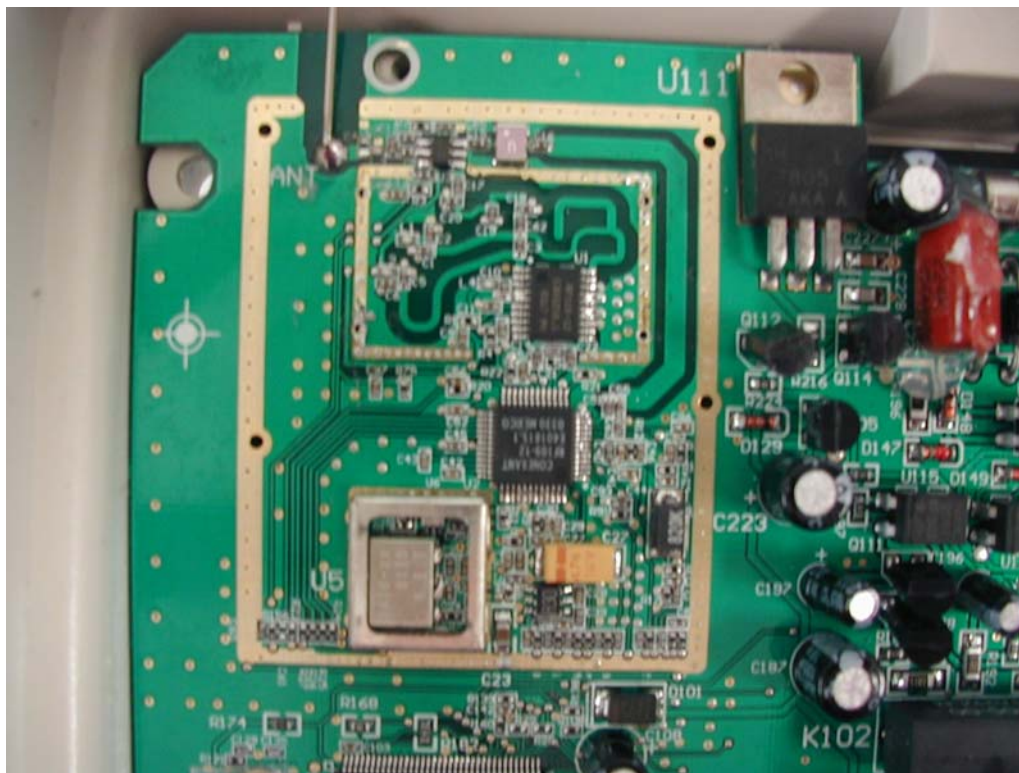
Figure 2: Base Unit – Main PCB Top View - without RF Circuit Covers
