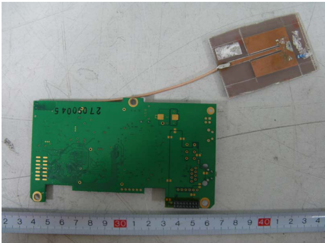
EUT-Module Rear View
