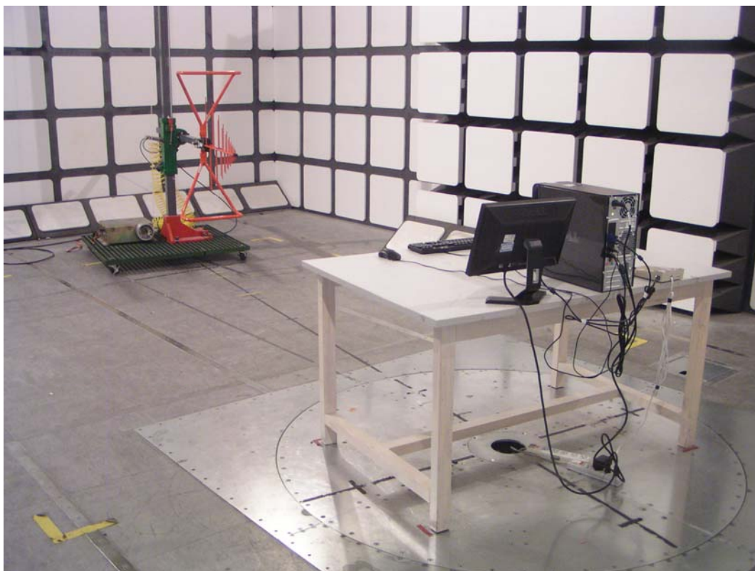
Radiated Emission - Rear View (30 -1000 MHz)
