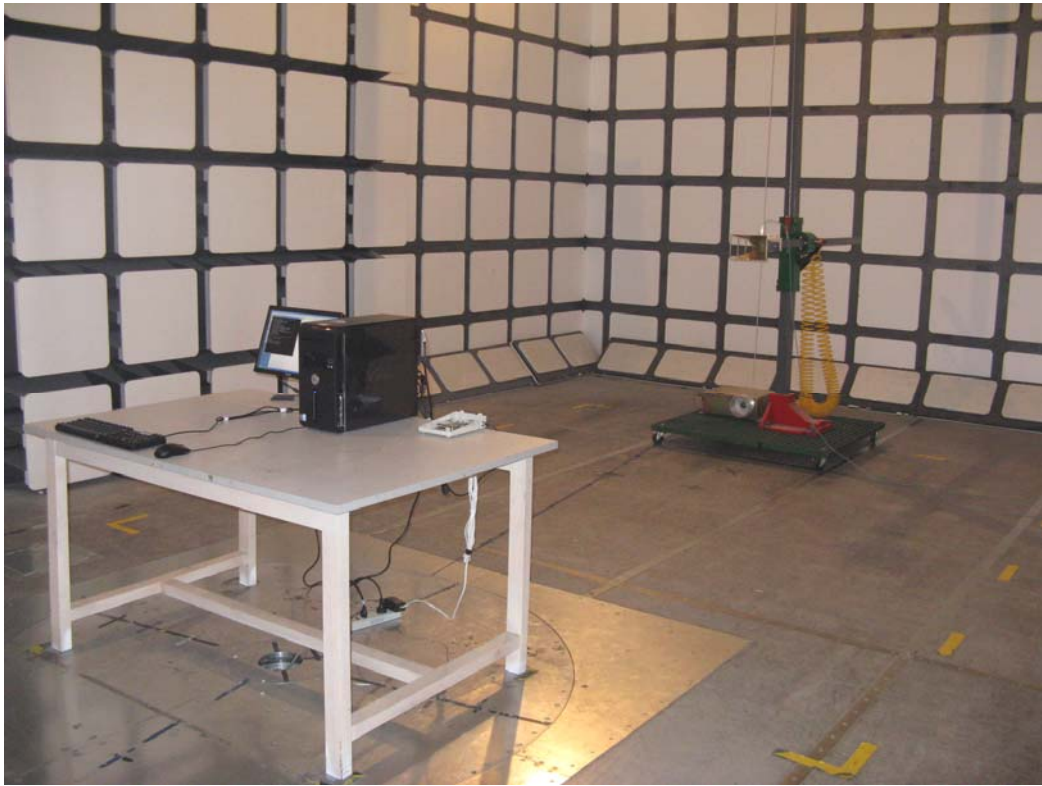
Radiated Emission - Rear View (Above 1 GHz)
