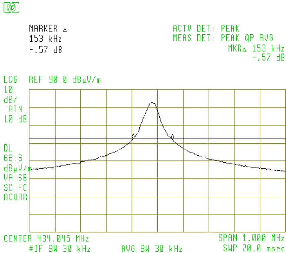
Figure 6.1 Occupied Bandwidth
