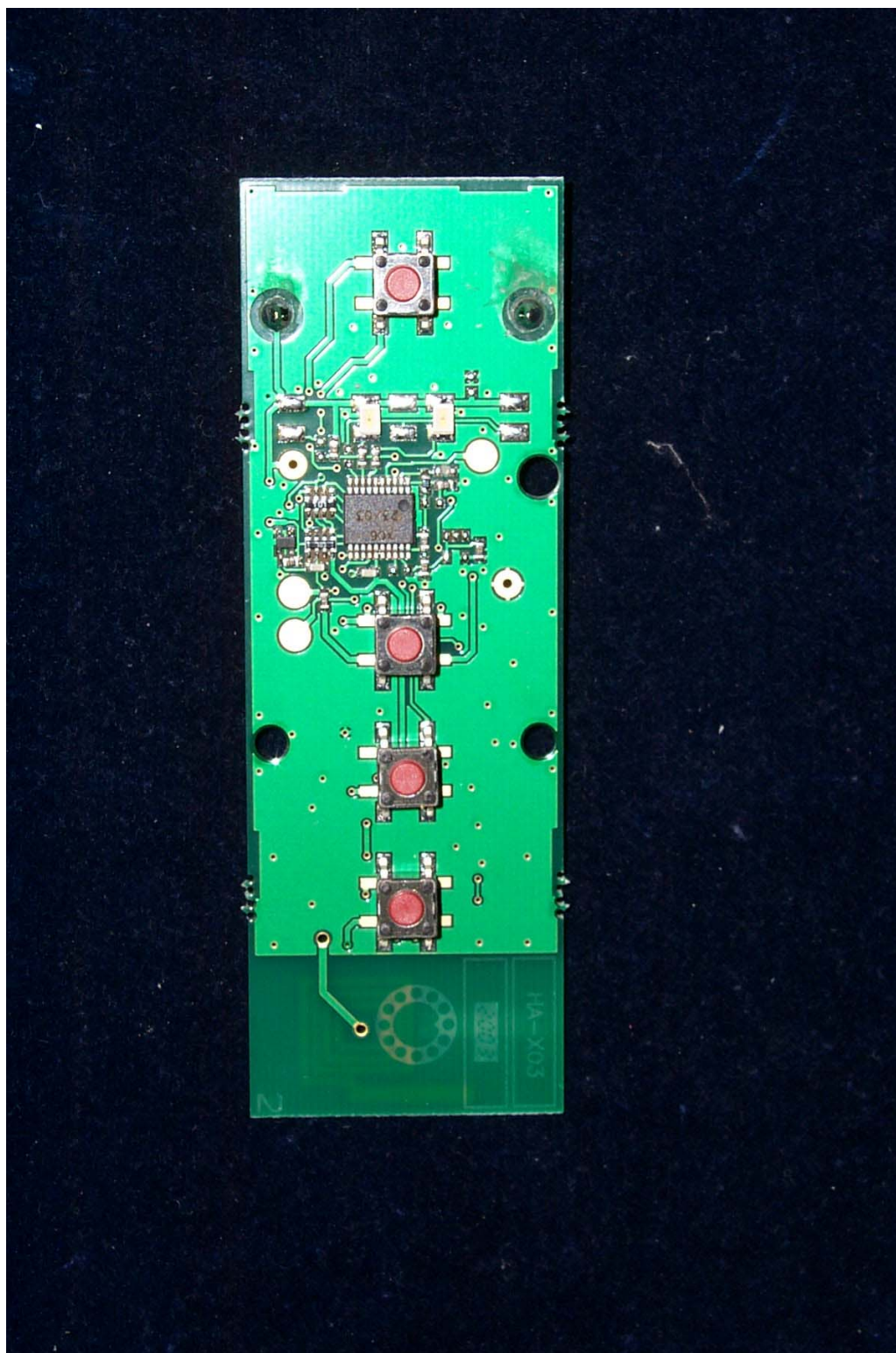
Figure 6.4 Component Side
