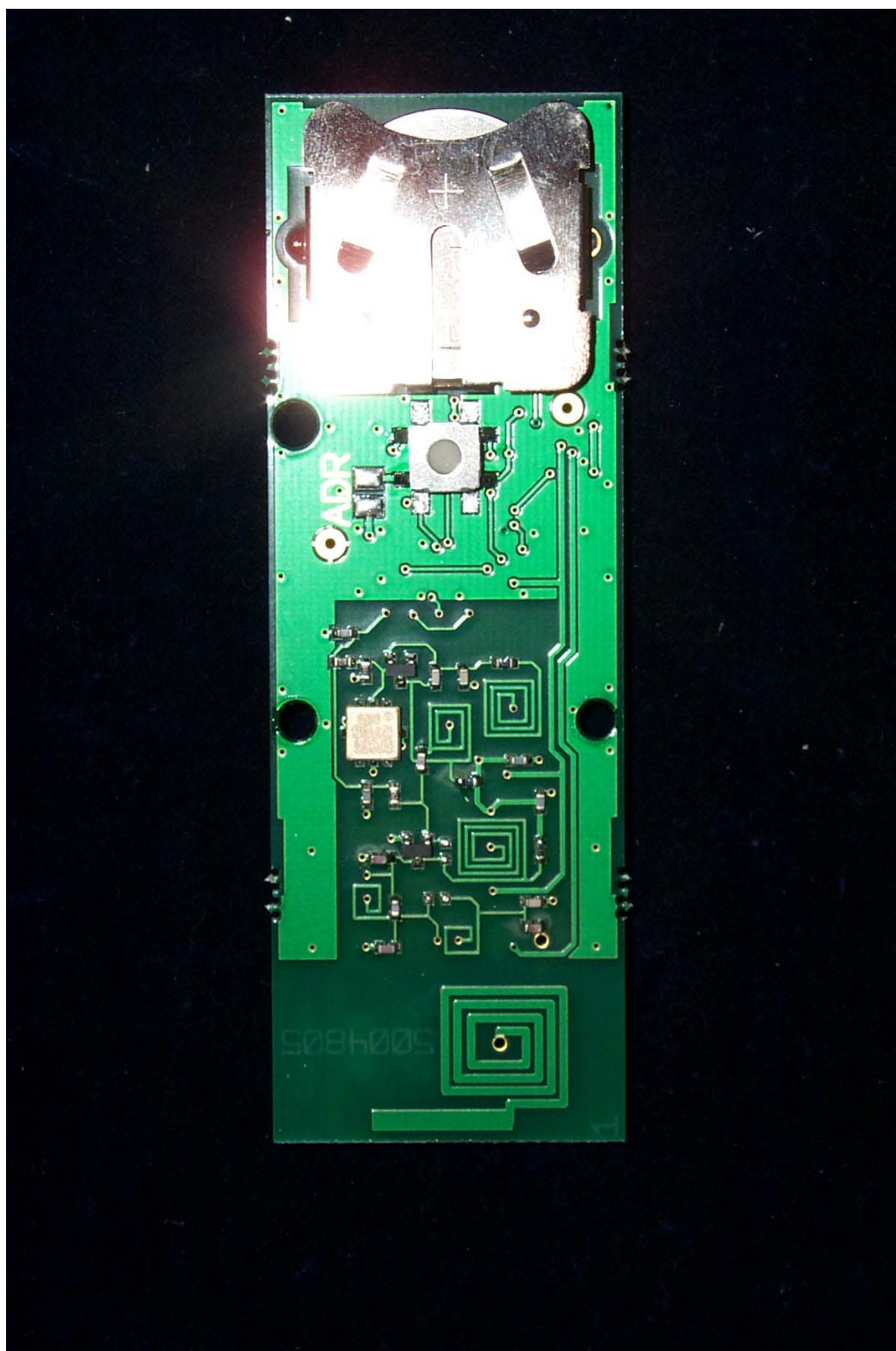
Figure 6.5 Foil Side
