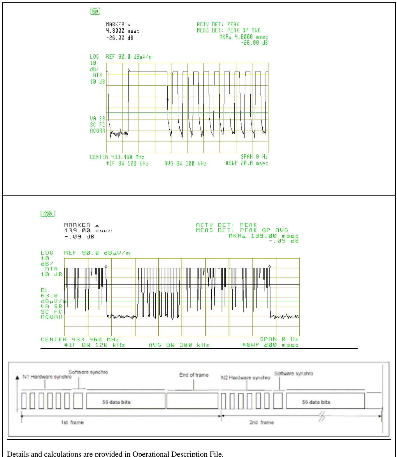
Figure 6.2 Pulse Train Timing
