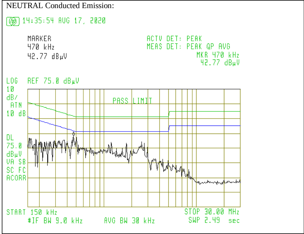
Figure 5.2 NEUTRAL Conducted Emission
