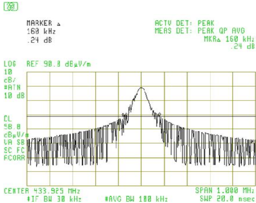
Figure 6.1 Occupied Bandwidth
