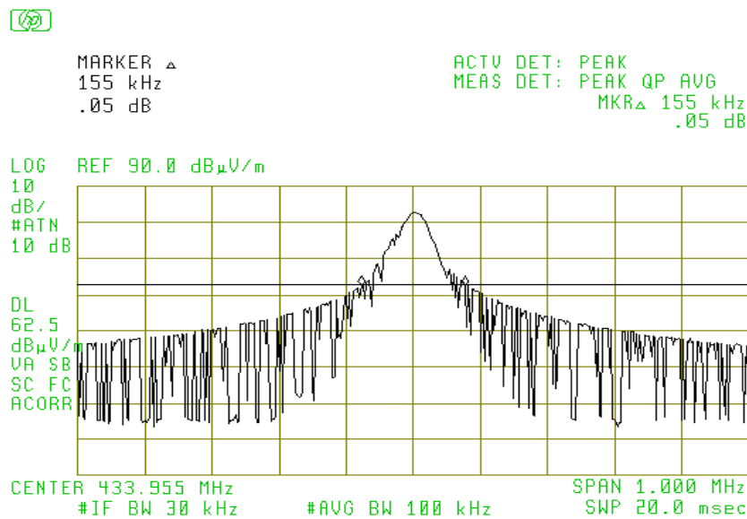
Figure 6.1 Occupied Bandwidth
