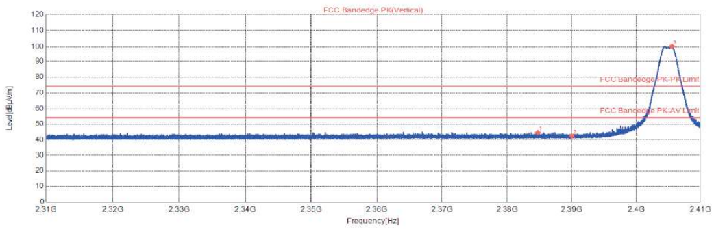
Zigbee_Ant1_2405 / Vertical
