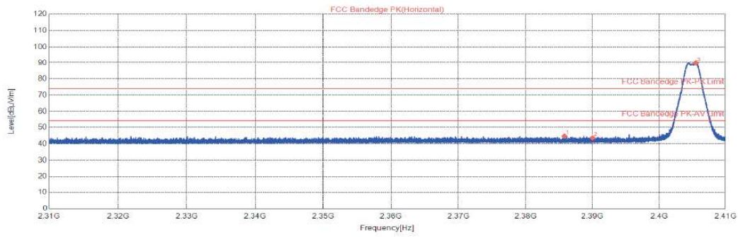
Zigbee_Ant1_2405 / Horizontal
